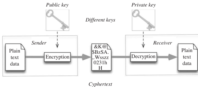
FIGURE 5.4 Asymmetric encryption.
