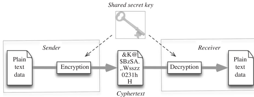
FIGURE 5.3 Symmetric encryption.
