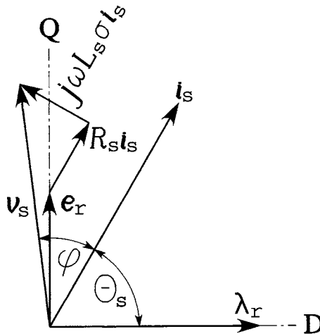
FIGURE 10.9 Vector diagram of a field-oriented induction motor.
