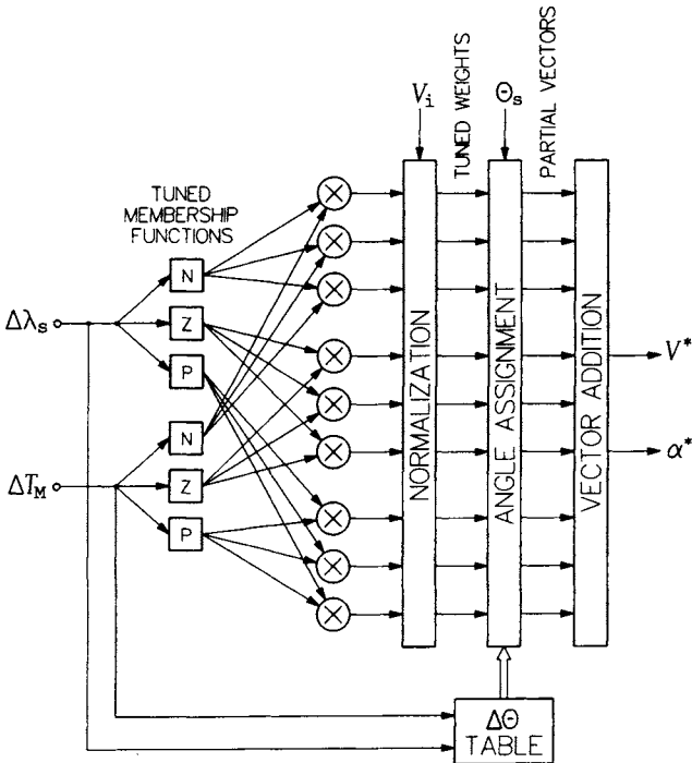
FIGURE 9.14 Neuro-fuzzy controller in Example 9.2.
