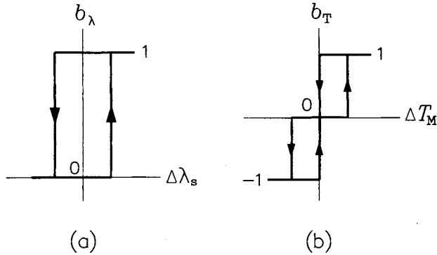
FIGURE 8.5 Characteristics of: (a) flux controller, (b) torque controller.
