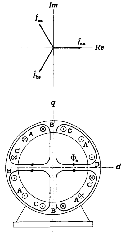
FIGURE 2.8 Phasor diagram of stator currents and the resultant magnetic field in a four-pole motor at \omega t = 0 .
