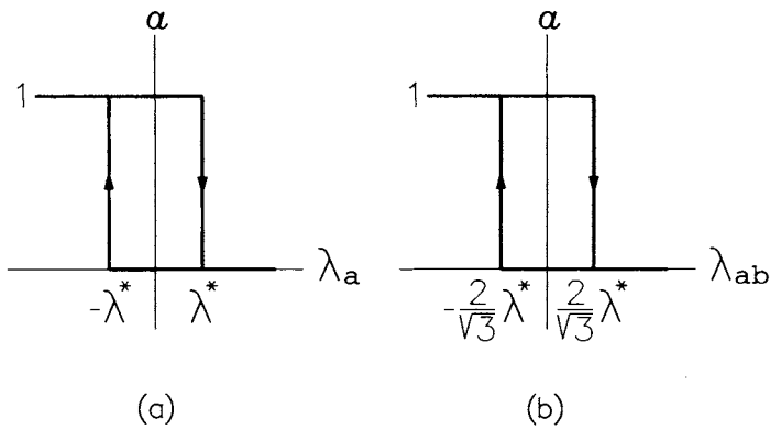
FIGURE 8.14 Characteristics of the hysteresis relays in the inverter self-control scheme: (a) line-to-neutral voltages integrated, (b) line-to-line voltages integrated.
