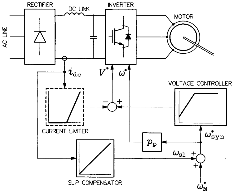
FIGURE 5.6 CVH drive system with slip compensation.
