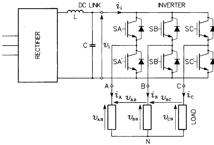
FIGURE 4.13 Voltage source inverter.
