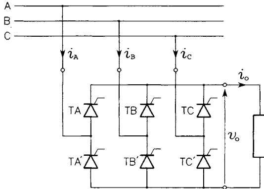
FIGURE 4.4 Six-pulse phase-controlled rectifier.
