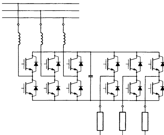
FIGURE 4.19 Current source PWM frequency changer.
