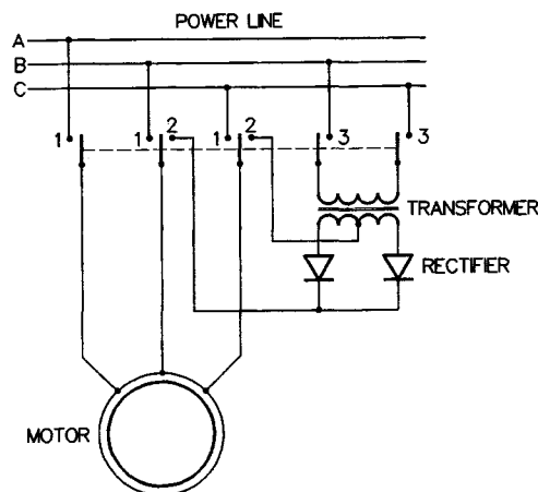
FIGURE 3.5 System for the dynamic braking.
