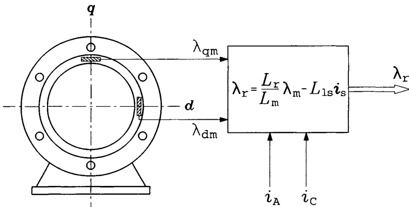
FIGURE 7.5 Estimation of the rotor flux vector based on direct measurements of the air-gap flux.
