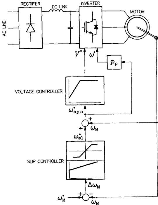
FIGURE 5.7 Scalar-controlled drive system with slip controller.
