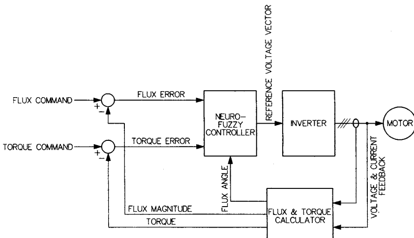
FIGURE 9.12 Block diagram of an SVTDC drive with neuro-fuzzy controller.
