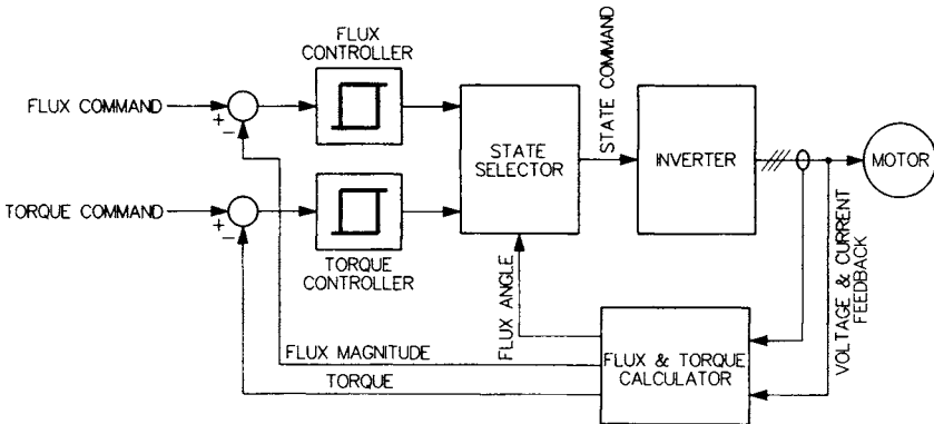
FIGURE 8.12 Simplified block diagram of the DTC scheme.
