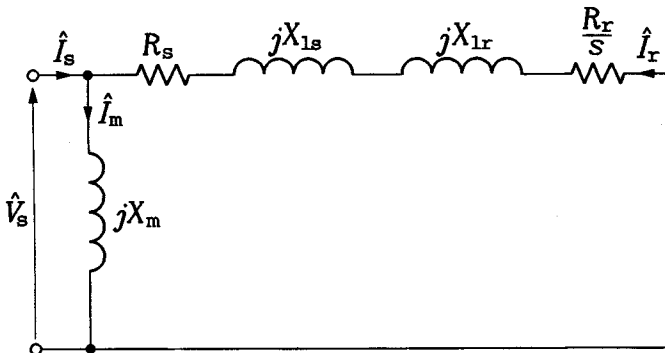
FIGURE 2.16 Approximate per-phase equivalent circuit of the induction motor.
