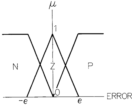
FIGURE 9.13 Membership functions of the flux and torque errors in Example 9.2.
