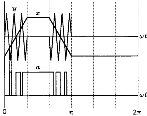
FIGURE 4.34 Illustration of a PWM technique for a current source inverter.
