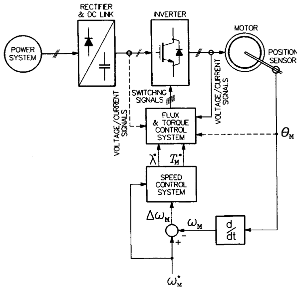
FIGURE 9.2 General block diagram of a high-performance adjustable speed drive.
