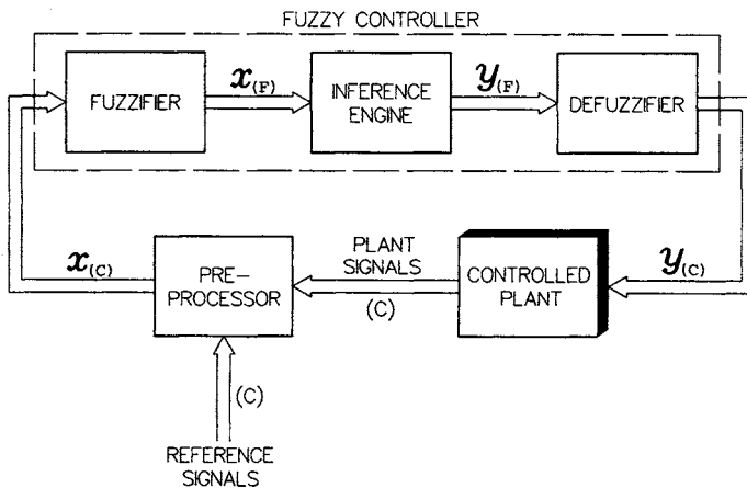
FIGURE 9.9 Block diagram of a fuzzy control system.
