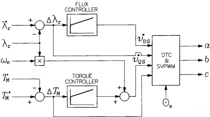
FIGURE 8.20 Block diagram of the core of SVDTC drive system.
