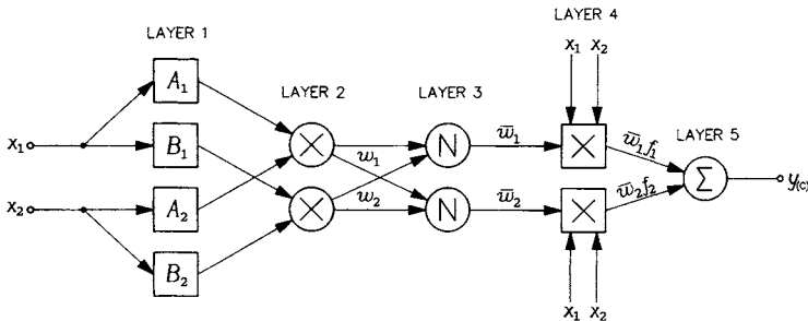
FIGURE 9.11 Neuro-fuzzy ANFIS controller.
