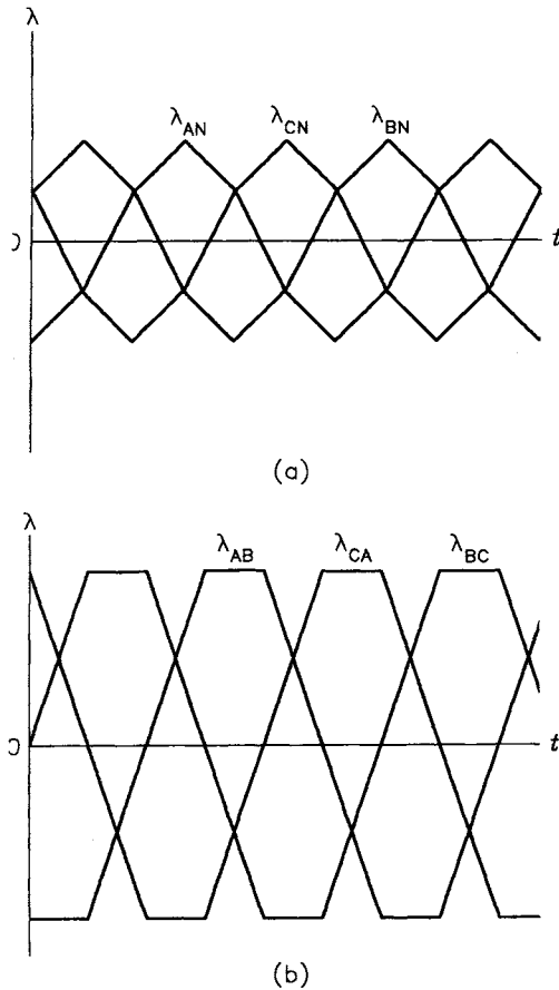
FIGURE 8.15 Waveforms of virtual fluxes: (a) line-to-neutral voltage integrals, (b) line-to-line voltage integrals.
