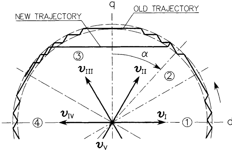
FIGURE 8.9 Acceleration of the stator flux vector by sector shifting.
