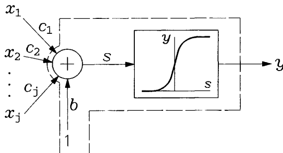
FIGURE 9.7 Single neuron.
