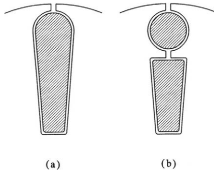
FIGURE 2.3 Cross-section of a rotor bar in (a) deep-bar cage, (b) double cage.
