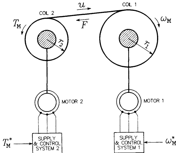
FIGURE 9.1 Winder drive system.
