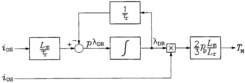
FIGURE 7.3 Block diagram of the field-oriented motor in a revolving reference frame aligned with the rotor flux vector.
