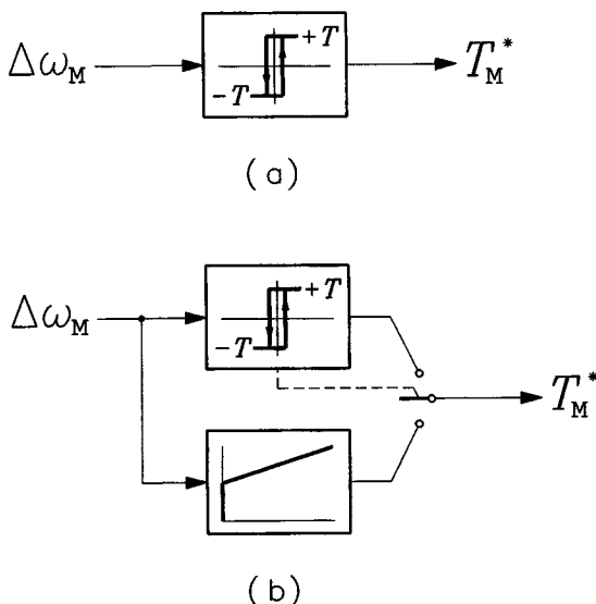
FIGURE 9.5 Variable-structure speed controllers: (a) relay, (b) relay/linear.
