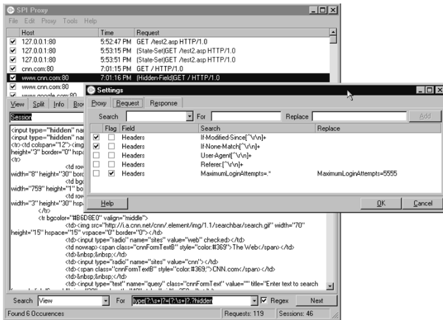
Figure B.14 Using SPI Proxy to Perform Automated Search and Replace of HTTP Elements
