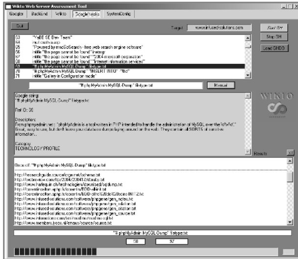
Figure 11.25 Wikto Manual Search Results
