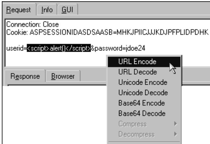
Figure B.18 HTTP Request Being Modified to Insert a Script
