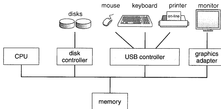
Figure 19.1 Bus-oriented organization.
