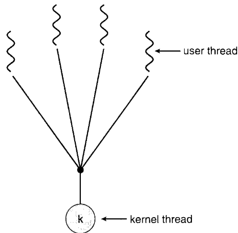
Figure 4.2 Many-to-one model.
