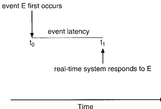
Figure 19.3 Event latency.
