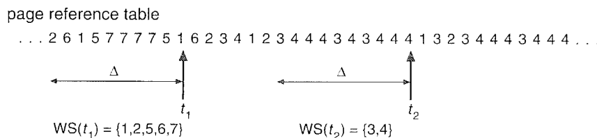
Figure 9.20 Working-set model.
