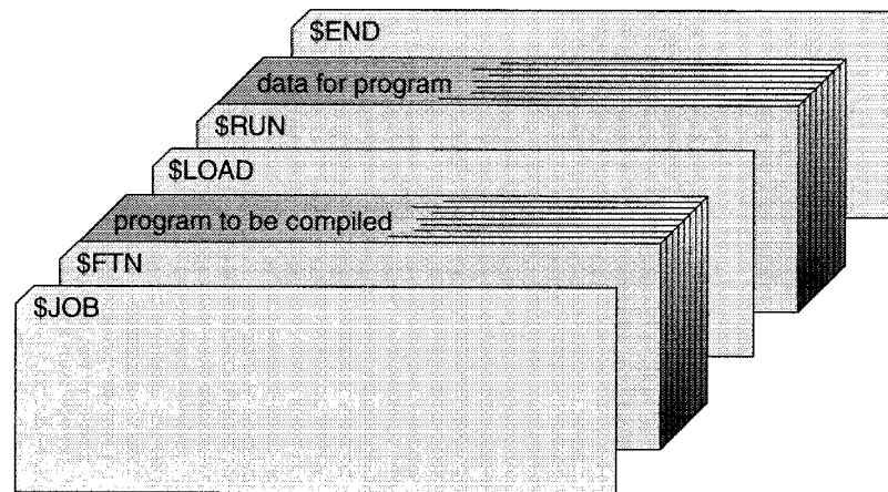
Figure 23.2 Card deck for a simple batch system.
