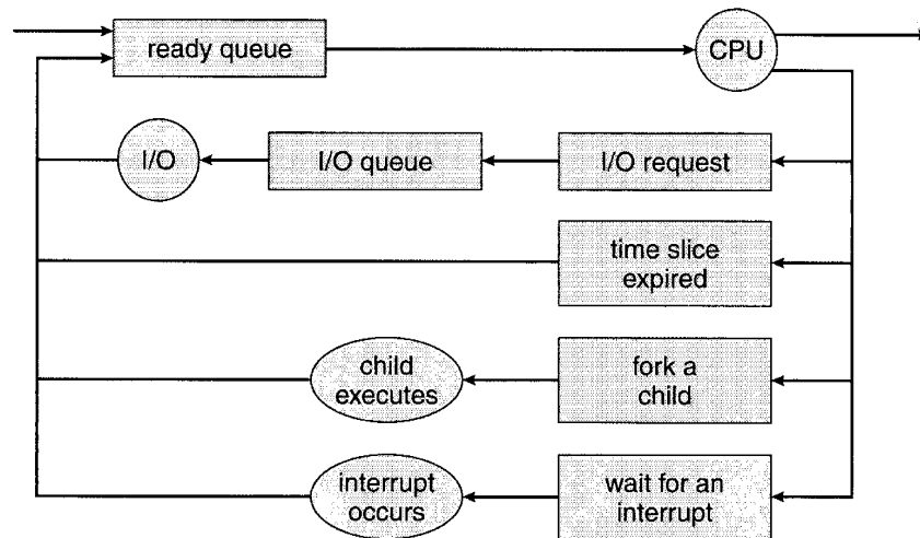
Figure 3.7 Queuing-diagram representation of process scheduling.
