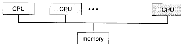
Figure 1.6 Symmetric multiprocessing architecture.
