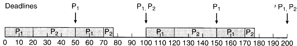
Figure 19.8 Rate-monotonic scheduling.
