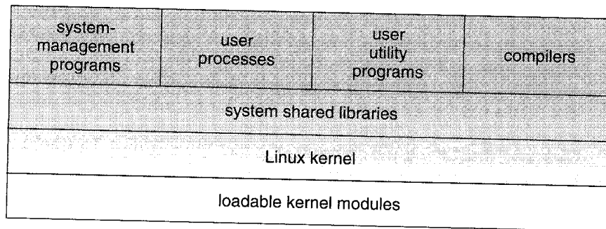
Figure 21.1 Components of the Linux system.
