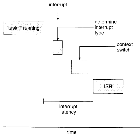
Figure 19.4 Interrupt latency.
