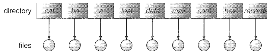
Figure 10.7 Single-level directory.
