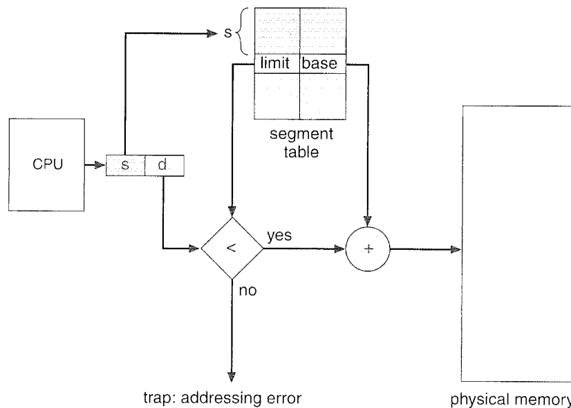
Figure 8.19 Segmentation hardware.
