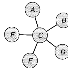
star network
