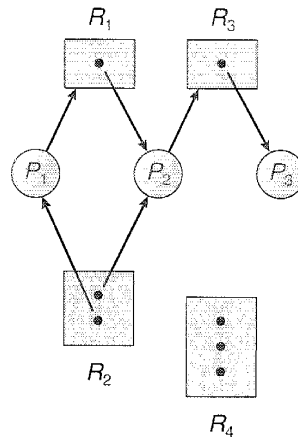
Figure 7.2 Resource-allocation graph.
