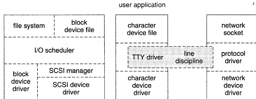
Figure 21.10 Device-driver block structure.
