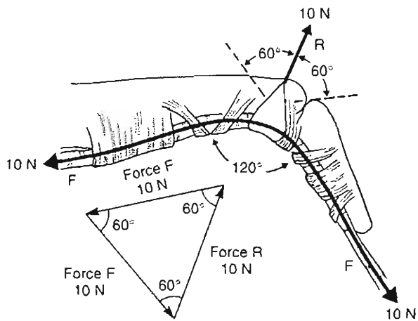
Calculation Box Figure 14-1-1. Lateral view. The PIP joint is flexed 60°. With the system in equilibrium, the resultant force (R) in the pulley system is equal to the vector sum of the two components of the tensile force (F) in the flexor tendon (i.e., 10 N). These three forces are presented graphically in an equilateral triangle of forces.
