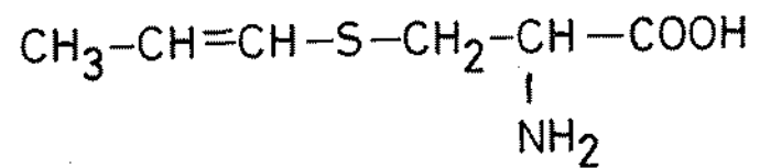
Propenyl - L - Cysteine (10)
