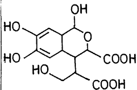
Chebulic acid (287)
