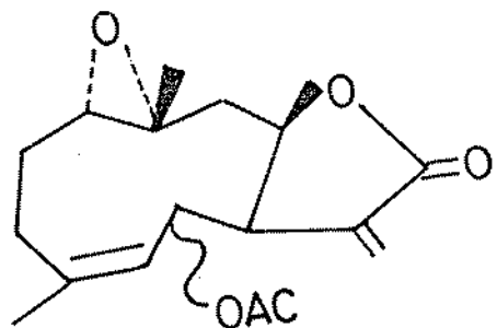
Pyrethrosin (75)
