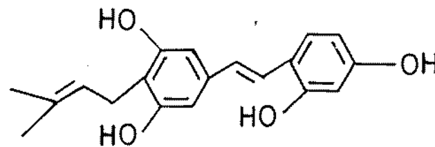
4 - Prenyloxyresveratrol (241)
