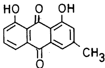
Chrysophanic acid (66)
