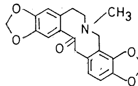
Protopine (162)
