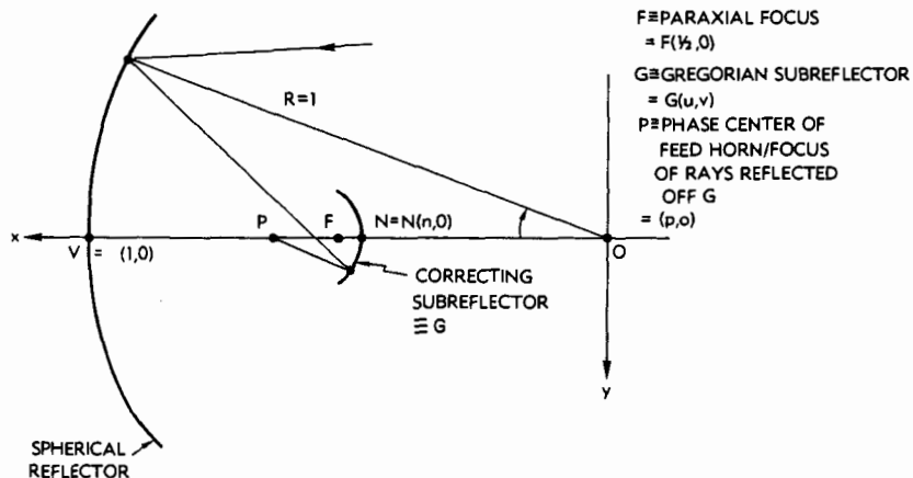
FIG. 17-45 Geometry of a gregorian correcting subreflector for a spherical reflector.
