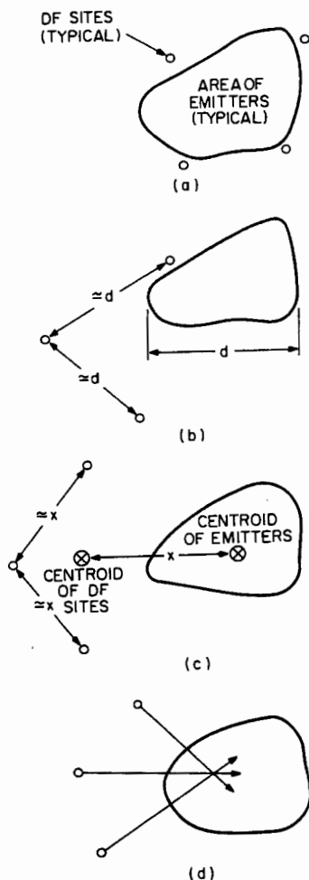
FIG. 39-7 Distribution of DF sites for minimum horizontal triangulation error. (a) Ideal distribution of DF sites. (b) Approach to ideal distribution of DF sites. (c) Optimum distribution if no DF site can be near the target area. (d) DF site location with respect to other fixed sites. Sites should be located on nonparallel baselines and as nearly in a triangle or a square as possible.
