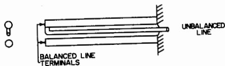
TYPE 10b THREE-WIRE BALUN
