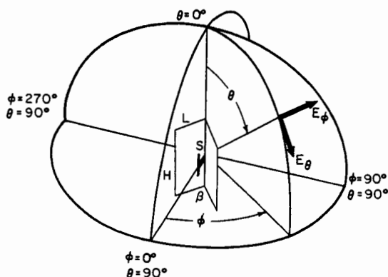
FIG. 17-1 Corner-reflector antenna and coordinate system.
