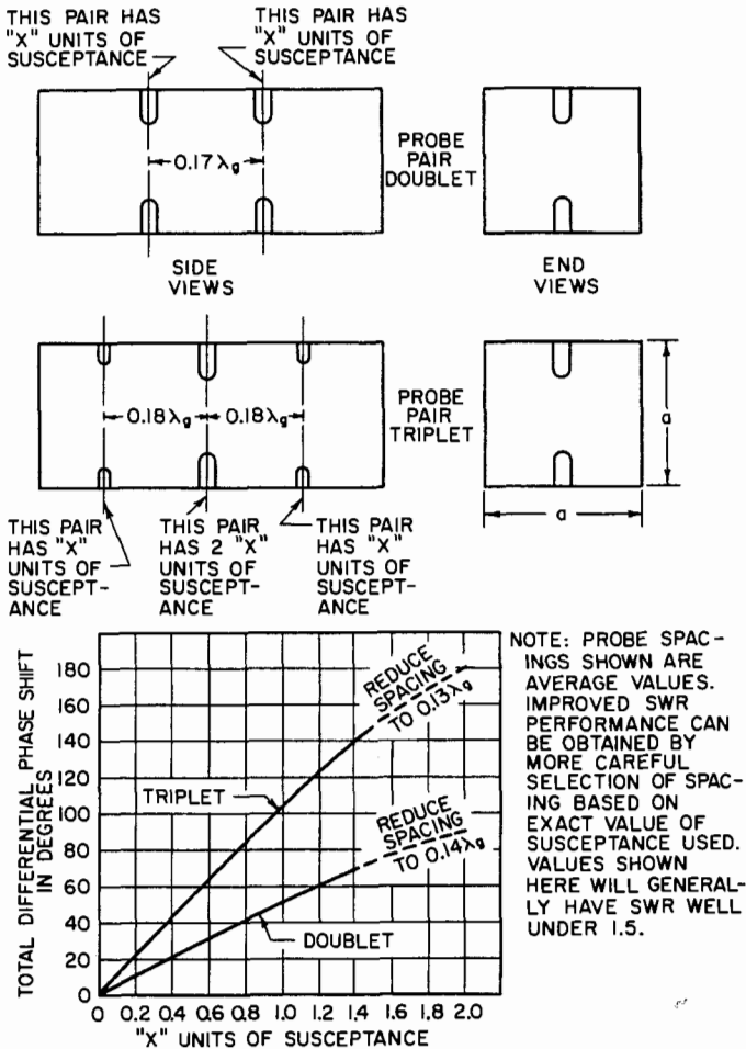
FIG. 23-27 Probe phase-shifter design.
