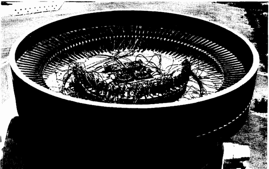
FIG. 21-9 Ring array. (After Boyns et al. 17 )
