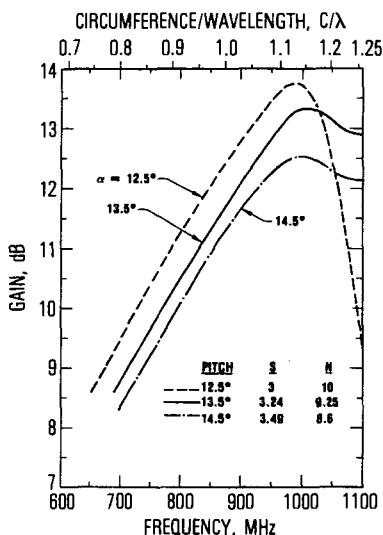
FIG. 13-6 Gain versus frequency of a fixed-length ( NS = 30 in, or 762 mm) helix; \alpha = 12.5^\circ, 13.5^\circ, and 14.5^\circ, D = 4.3 in, or 762 mm); \alpha = 12.5^\circ, 13.5^\circ, and 14.5^\circ, D = 4.3 in (109 mm).
