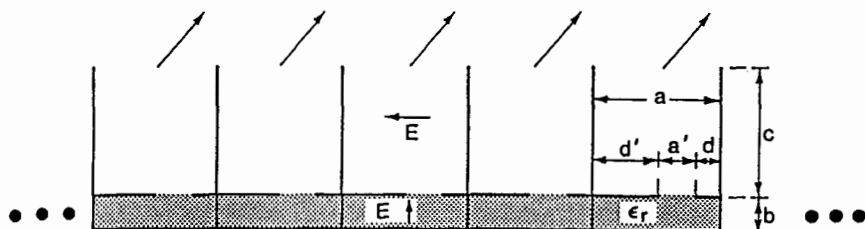
FIG. 10-38 Cross section of the linear phased array of printed-circuit uniform leaky-wave line sources. The individual line source appears in Fig. 10-31. (From Lampariello and Oliner. 69 )
