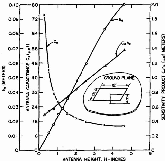
FIG. 37-4 Design data for a heavily top-loaded low-frequency antenna with flat-plate top loading.
