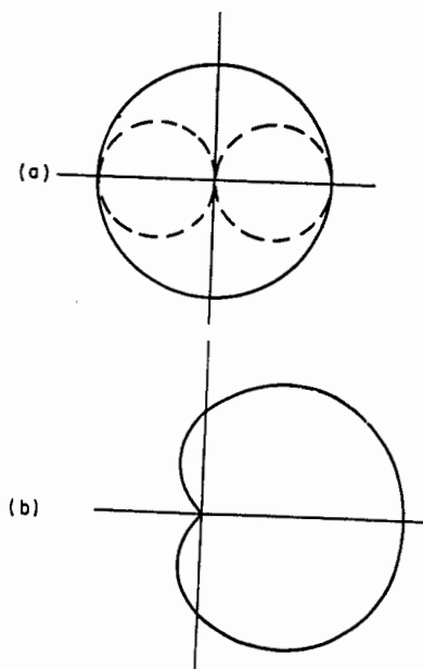
FIG. 2-9 Radiation patterns in plane of electric current loop. (a) ——— Pattern of electric current loop. ---- Pattern of electric dipole. (b) Cardloid pattern due to combination of electric current loop and electric dipole.
