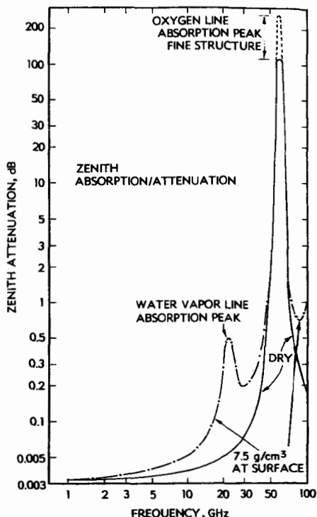
FIG. 45-3 Zenith absorption.
