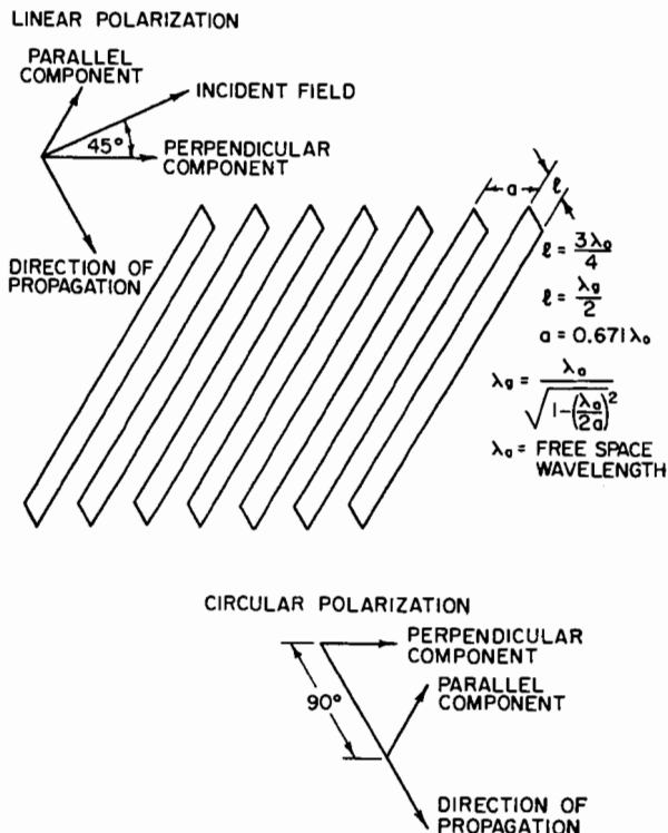
FIG. 23-31 Parallel-plate polarizer.
