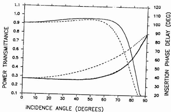
FIG. 44-8 Power transmittance (upper curves) and insertion phase delay versus incidence angle for an A-sandwich panel having a core design angle of 50^\circ for parallel (solid curve) and perpendicular (dash) polarizations ( \epsilon_{rs} = 4.0 , \tan \delta_s = 0.020 , d_s = 0.025\lambda , \epsilon_{rc} = 1.2 , \tan \delta_c = 0.005 , d_c = 0.293\lambda ).
