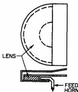
FIG. 18-13 Pillbox-concentric-lens system.
