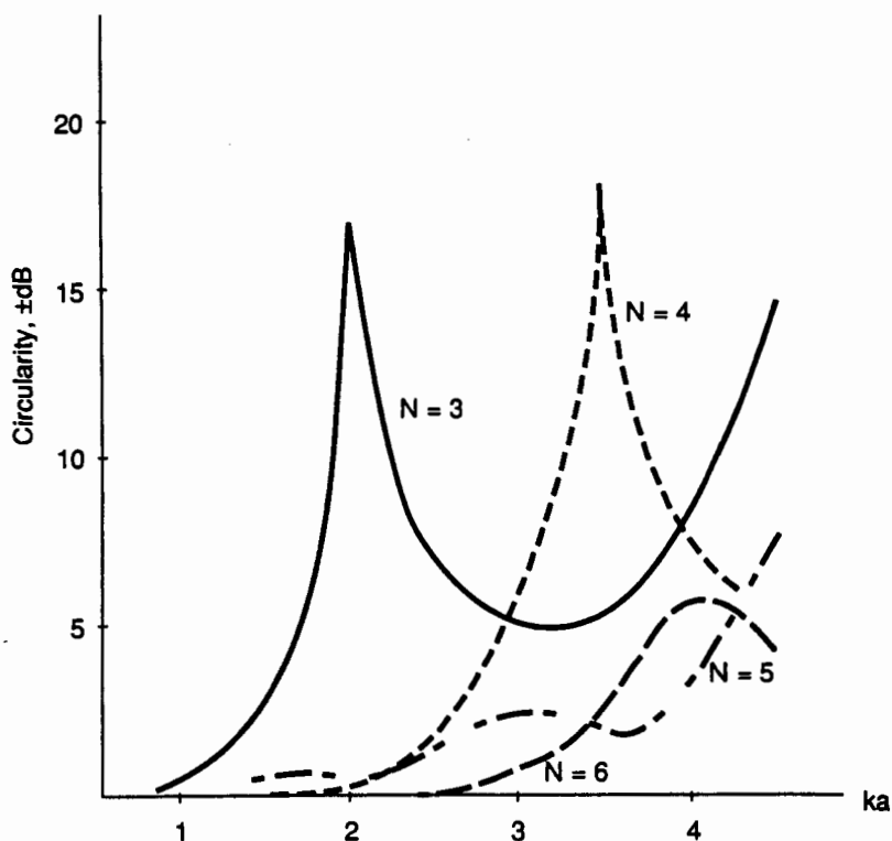
FIG. 28-34 Azimuth pattern circularity versus ka .
