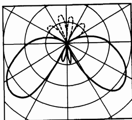
QUARTER-WAVE STUB
