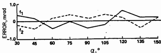
FIG. 34-25 \alpha - \alpha_1 error with scan angle.
