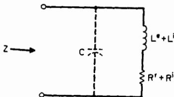
FIG. 5-3 Equivalent circuit for input impedance Z of an electrically small loop.
