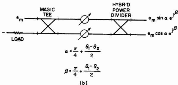
FIG. 22-4 (a) RF weight circuit. (b) Variable power-divider circuit.
