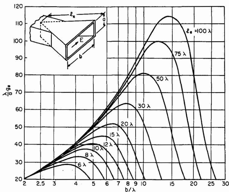
FIG. 15-6 Gain of E -plane sectoral horn ( a \leq \lambda ).
