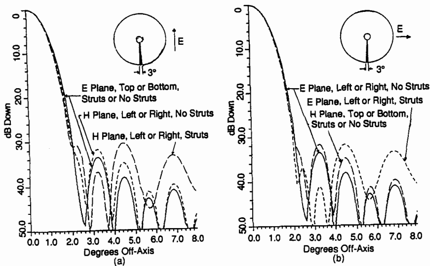
FIG. 30-22 Predicted effects on near on-axis dish patterns due to strut blockage ( D = 12 ft, MD feed, F/D = 0.400 , f = 3.95 GHz, 1.2-in-diameter strut, modeled by 3^\circ strut).
