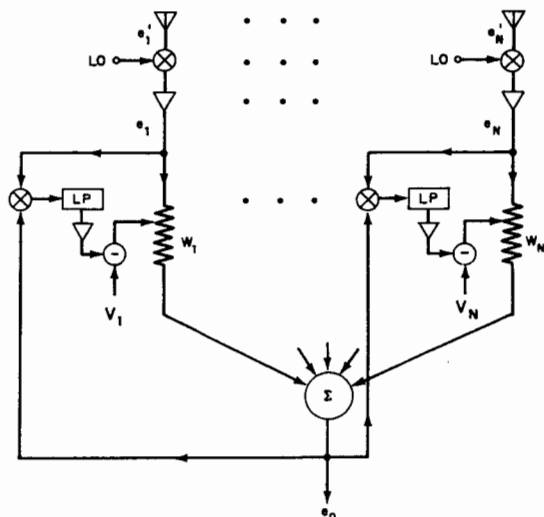
FIG. 22-10 Applebaum-Howells circuit.
