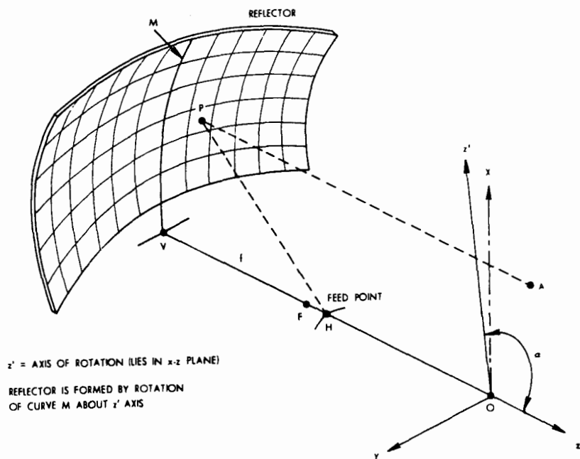
FIG. 17-46 Torus-antenna geometry.
