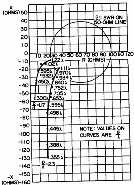
FIG. 37-29 Impedance of an annular-slot antenna.
