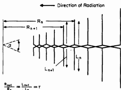
FIG. 26-3 Basic half-wave transposed dipole LPA.
