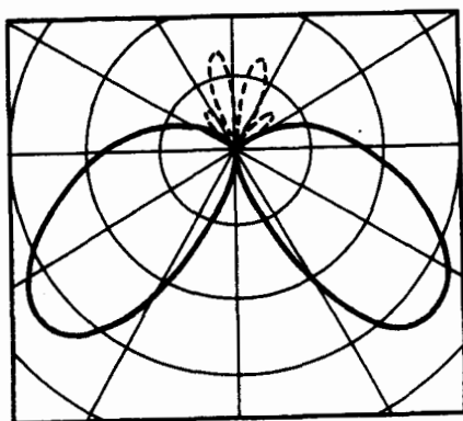
SLOT APERTURE DIAMETER = 0.6\lambda
