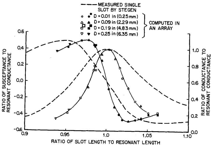
FIG. 9-11 Admittance of the baseline longitudinal shunt slot versus normalized resonant slot length. The solid curves are best fit to the computed points.
