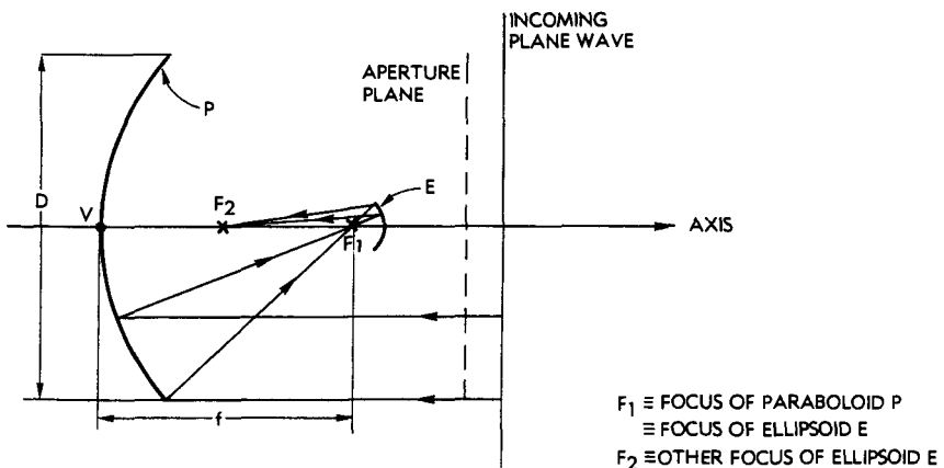
FIG. 17-34 Gregorian geometry.
