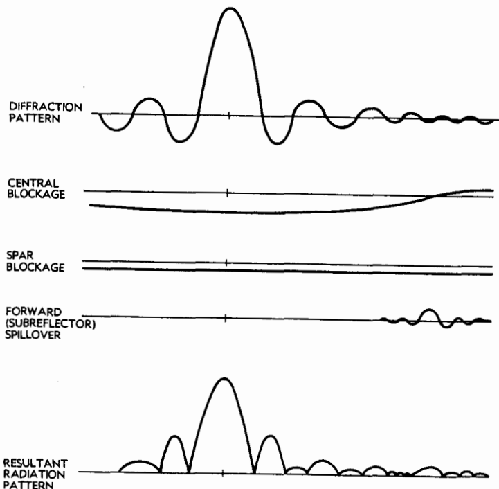
FIG. 17-37 Blockage effects on sidelobe structure.
