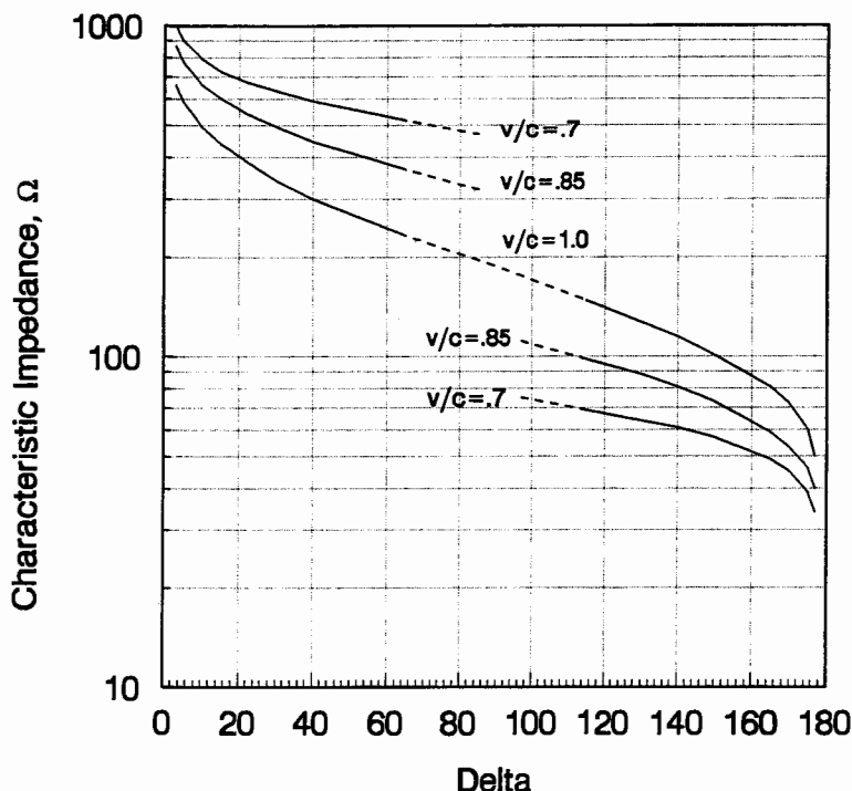
FIG. 14-12 Log-spiral input impedance versus \delta for v/c = 0.7, 0.85, and 1.0 and \tau = 0.4 .
