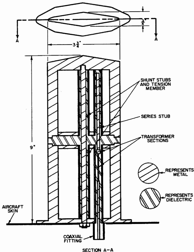
FIG. 37-27 The AT-256A antenna.
