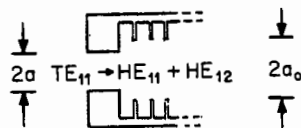
FIG. 15-36 Two-hybrid-mode generation at a step discontinuity.
