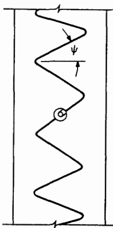
FIG. 28-31 Zigzag antenna with balanced feed.
