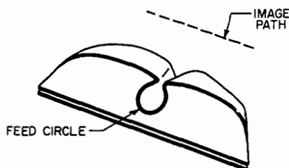
FIG. 18-21 Robinson scanner.
