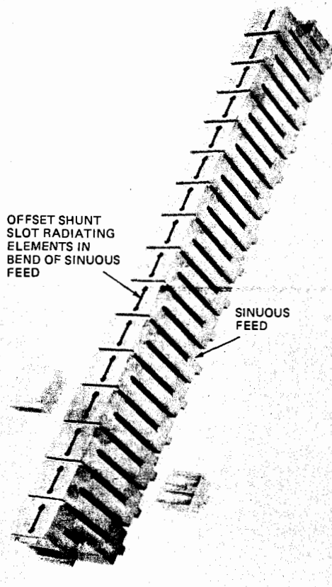
FIG. 19-15 Waveguide sinuous feed with offset shunt-slot radiators.
