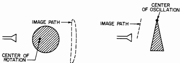
FIG. 18-24 Prism scanners.
