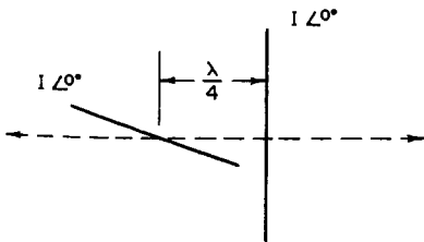
FIG. 23-16 Crossed dipoles—current in phase— \lambda/4 separation.
