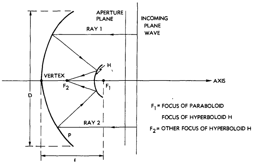
FIG. 17-33 Cassegrain geometry.
