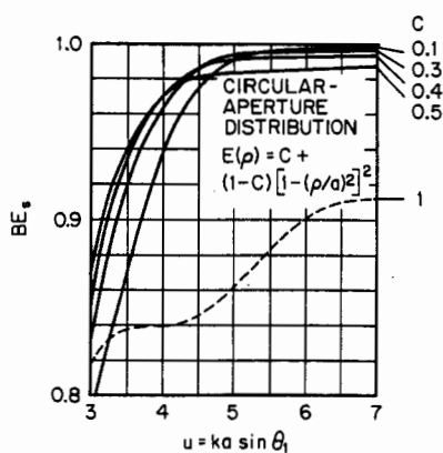
FIG. 31-11 Beam efficiency for circular aperture with a parabola-on-a-pedestal-squared distribution.
