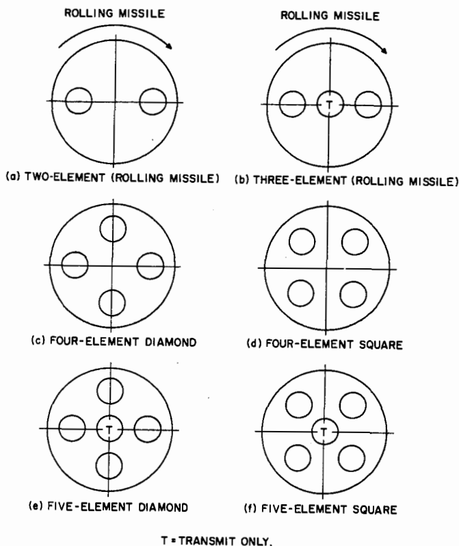
FIG. 38-8 Small-array geometries.
