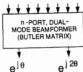
FIG. 39-17 Dual-mode antenna array and beamformer.
