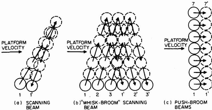
FIG. 31-8 Ground spot patterns of radiometer-antenna systems.
