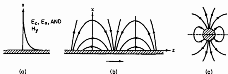
FIG. 12-4 Surface-wave field structure above interface. (a) TM-wave components on plane surface. (b) Composite electric field lines over a one-wavelength interval (arrow points in the direction of propagation). (c) Composite electric field lines of HE_{11} wave on an axial-cylindrical surface (cross section). Dashed line shows the electric-image plane (Sec. 12-4).
