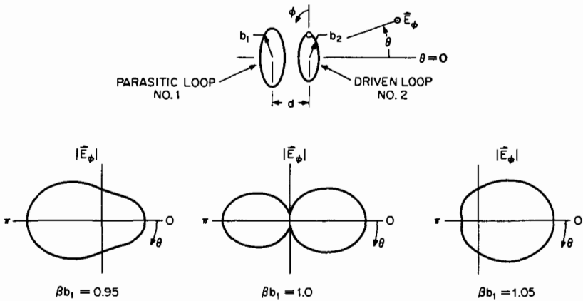
FIG. 5-20 Far-zone electric field patterns |\vec{E}_\phi| in plane \phi = 0, \pi for driven loop with single parasite, \beta b_2 = 1.0 , d/\lambda = 0.1 , \Omega_1 = \Omega_2 = 20 .
