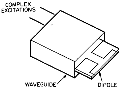
FIG. 23-14 Slot-dipole element.
