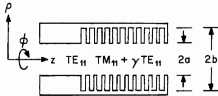
FIG. 15-23 Cylindrical corrugated waveguide with TE_{11} -mode excitation.
