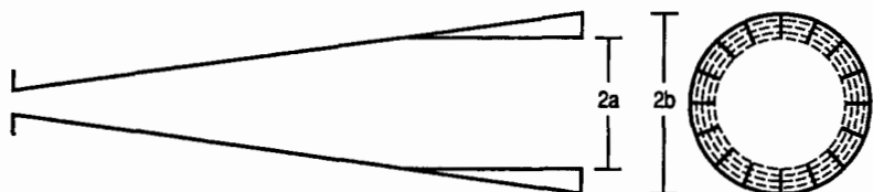
FIG. 15-38 Geometry of longitudinally slotted horn with dielectric in slots.
