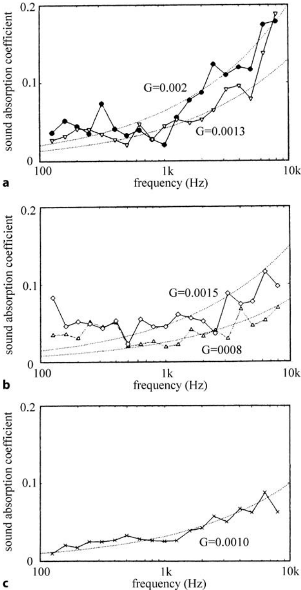
Fig. 4.29. Sound absorption coefficient for trees of different species and different leaves versus frequency (Watanabe and Yamada 1996). Reprinted with permission of the Acoustical Society of Japan, copyright 2005. \Delta Sawara cypress ( Chamaecyparis pisifera var. plumosa ), \bullet Japanese aucuba ( Aucuba japonica ), \diamond Japanese cedar ( Cryptomeria japonica ), \nabla spindle tree ( Euonymus japonica )
