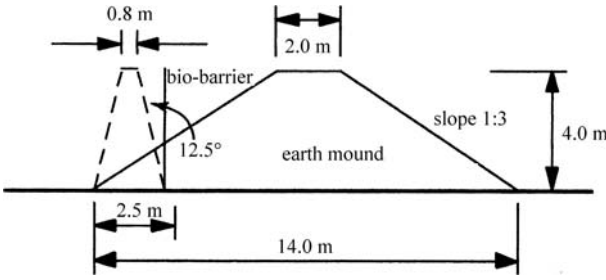
Fig. 4.54. Comparison between bio-barrier and earth mound of the same height (4 m) and of different wide (2.5 m for the bio-barrier and 14 m for the earth mound; Kotzen 2004)
