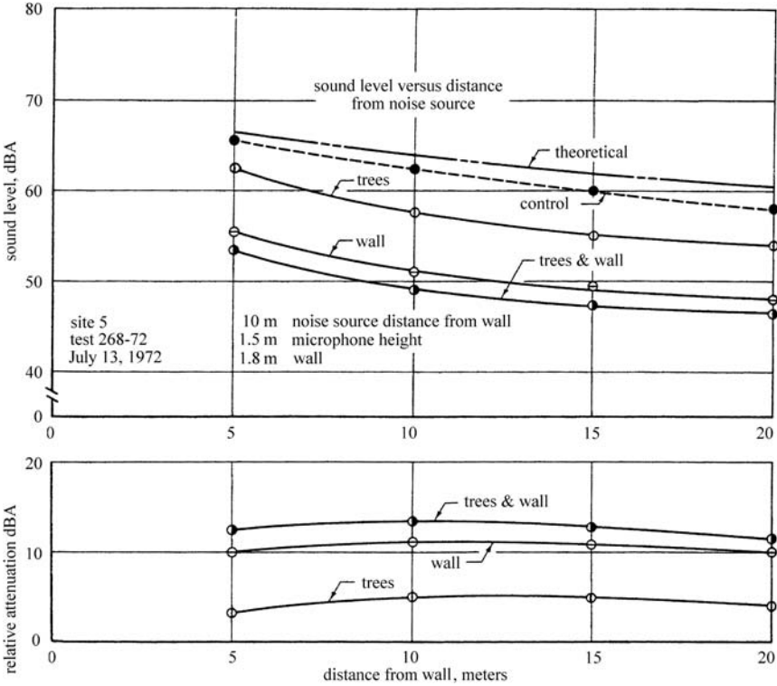
Fig. 6.8. The influence of different surfaces – wall alone, trees alone, trees and wall – on noise reduction (Cook and van Haverbeke 1972)
