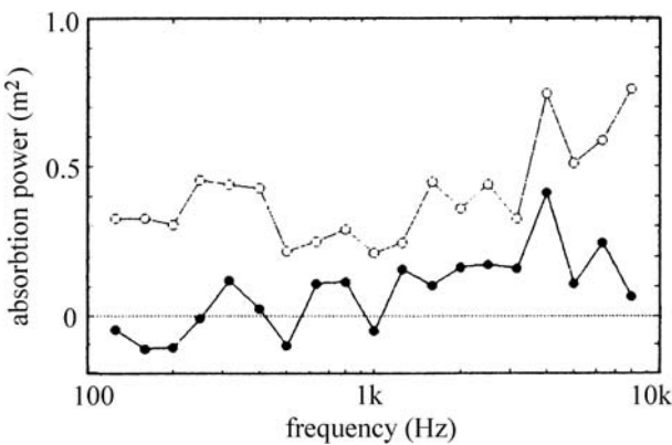
Fig. 4.28. Absorption power versus frequency for sawara cypress with and without leaves (Watanabe and Yamada 1996). \circ With leaves, surface 8.70 m 2 , \bullet without leaves. Reprinted with permission of the Acoustical Society of Japan, copyright 2005
