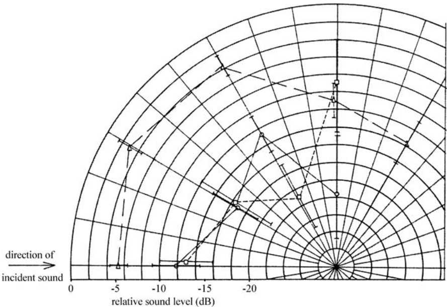
Fig. 4.36. Relative sound level (dB) of sound scattered by trees (Bullen and Fricke 1982). Reprinted with permission from Elsevier, copyright 2005. Circles Palm without important foliage, squares palm with foliage, triangles fig. The direction of the incident sound was between 0^\circ and 90^\circ
