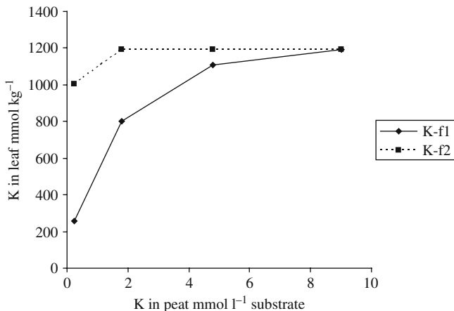
Fig. 11.5 The relationship between the K added to the peat substrate before planting and the K concentration in tomato leaves 8 weeks after planting at two levels of top dressing (Adams 2002). The levels of the top dressing were K-f1 = 2.6 mmol l -1 and K-f2 = 7.7 mmol l -1 . After Adams (2002). Modified after permission of Embryo Publications.
