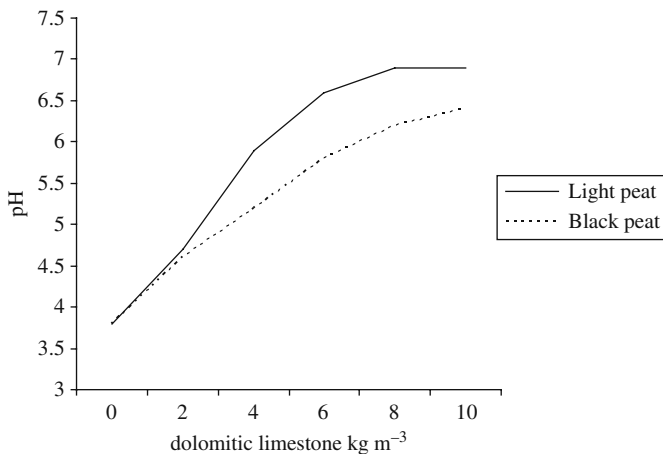
Fig. 11.2 The effect of the addition of lime on the pH of high more peat. After Van Schie (1989)
