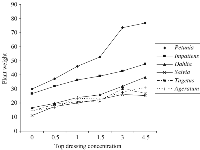
Fig. 14.1 Relationship between the concentration of the top dressing solution in g l -1 17-6-18 and the plant weight of a series of bedding plants. Data after Boertje (1980). Modified by permission of the International Society Horticultural Science
