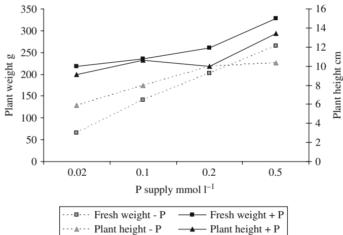
Fig. 14.6 Plant weight and plant height as affected by the P supply in the nutrient solution supplied with Pelargonium with and without P in the base dressing in the substrate. After Warmenhoven and van Noort (2005)
