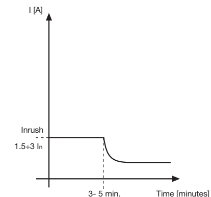
Inrush current diagram
