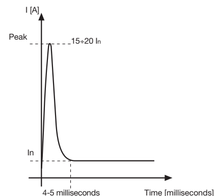
Peak current diagram
