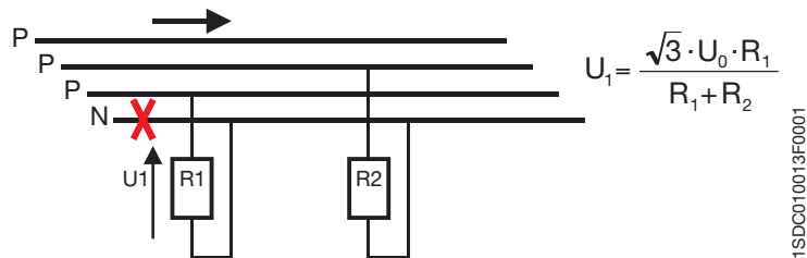
Figure 1: Disconnection of the neutral conductor
