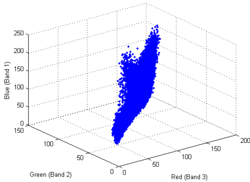
Color Scatterplot Before (left) and After (right) Decorrelation Stretch
