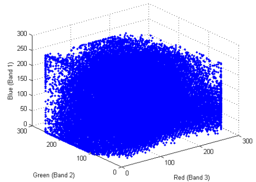
Color Scatterplot Before (left) and After (right) Decorrelation Stretch
