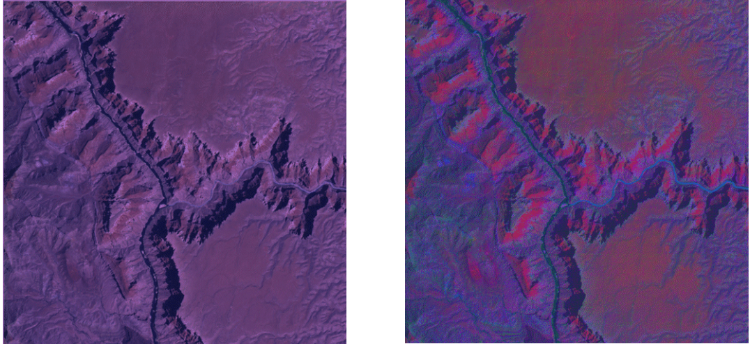
Little Colorado River Before (left) and After (right) Decorrelation Stretch
