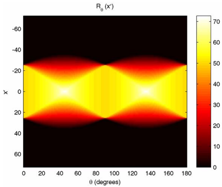
Radon Transform Using 180 Projections
