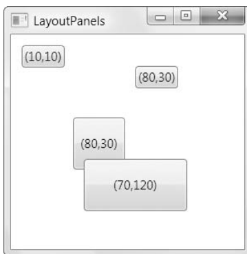
Figure 4-17. Explicitly positioned buttons in a Canvas
