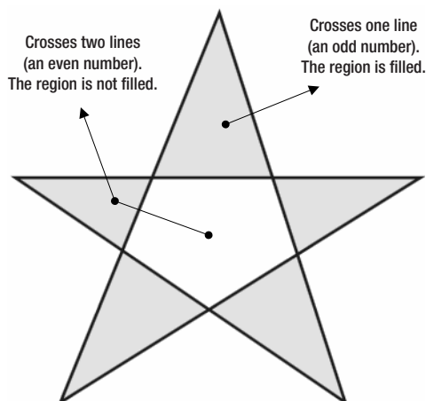
Figure 13-9. Determining fill areas when FillRule is EvenOdd
