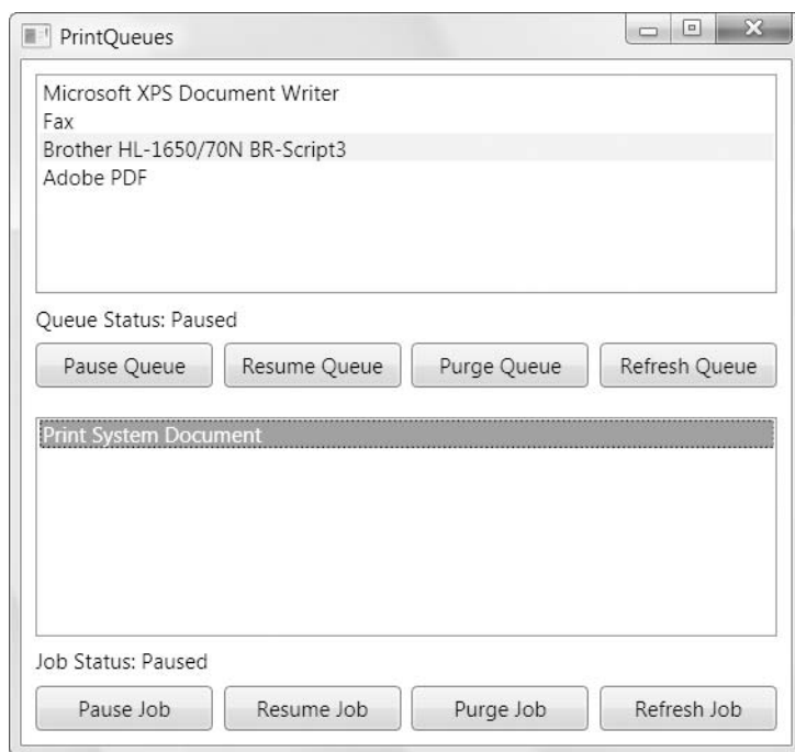
Figure 20-8. Browsing printer queues and jobs
