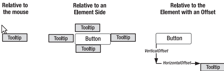
Figure 7-4. Placing a tooltip explicitly
