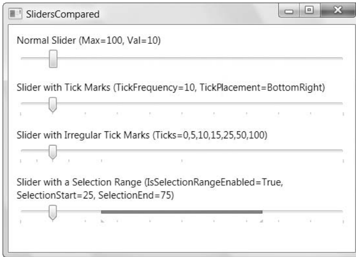
Figure 7-10. Adding ticks to a slider
