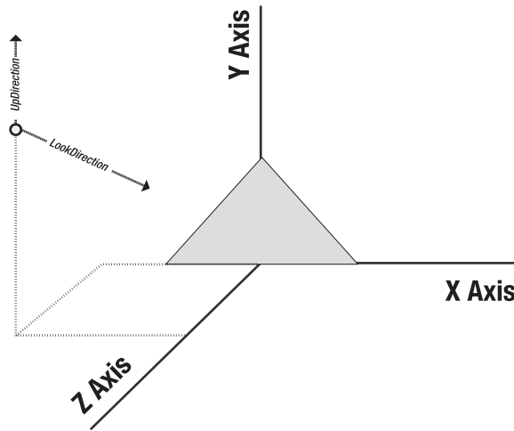
Figure 23-5. Positioning and angling the camera
