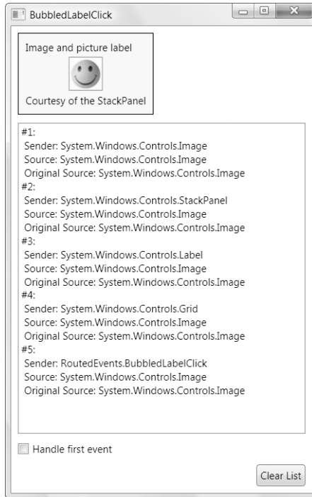
Figure 6-1. A bubbled image click
