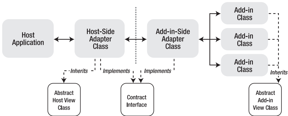
Figure 26-5. Multiple add-ins that use the same pipeline
