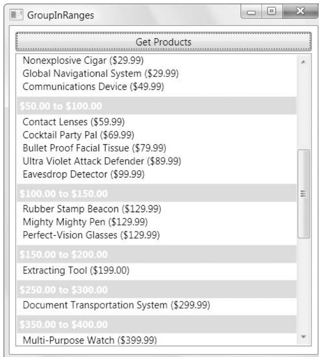
Figure 17-13. Grouping in ranges
