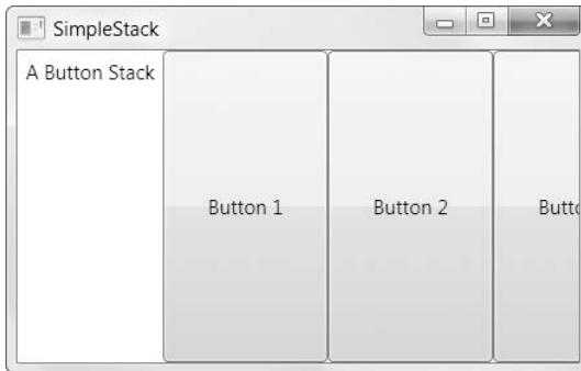
Figure 4-3. The StackPanel with horizontal orientation
