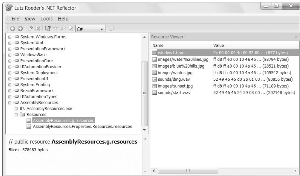
Figure 11-2. Assembly resources in Reflector
