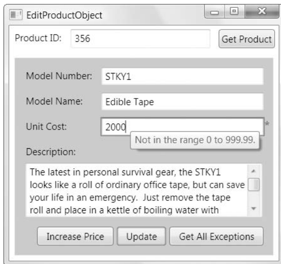
Figure 16-14. Turning a validation error message into a tooltip
