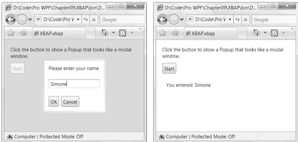
Figure 9-16. Simulating a dialog box with the Popup
