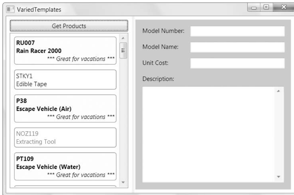
Figure 17-5. A list with two data templates
