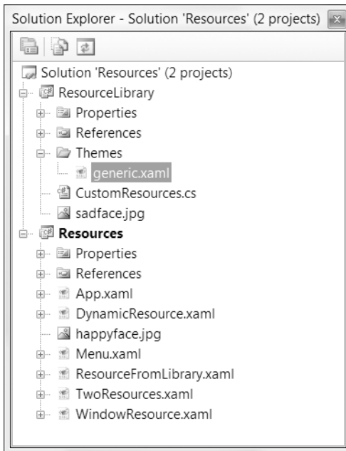
Figure 11-8. Sharing resources with a class library
