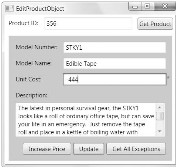
Figure 16-13. Flagging an error with an error template
