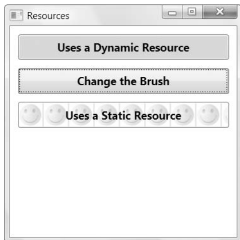
Figure 11-7. Dynamic and static resources
