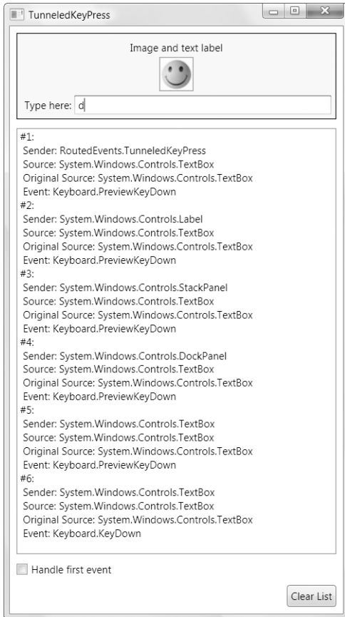
Figure 6-4. A tunneled key press
