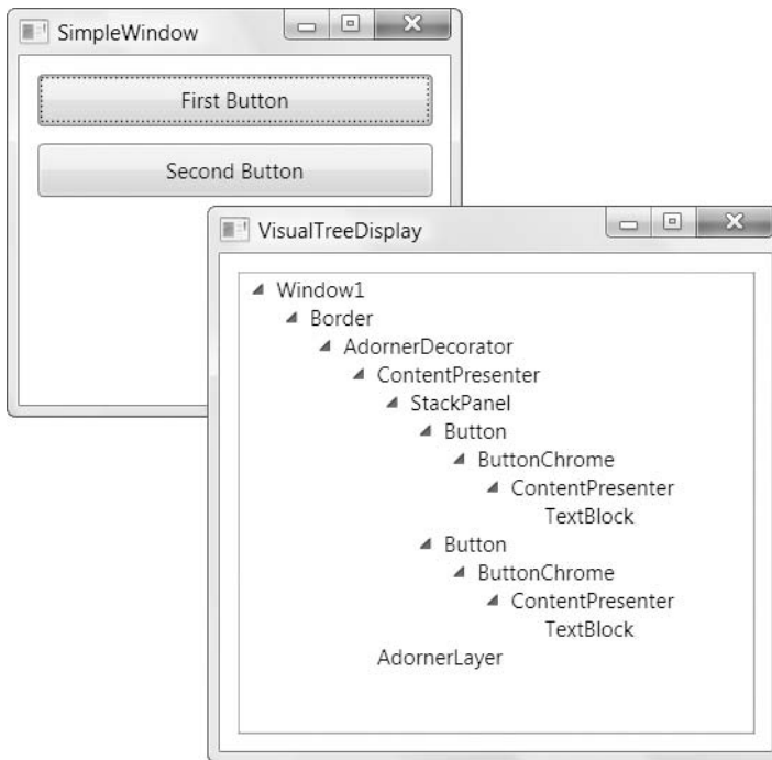
Figure 15-4. Programmatically examining the visual tree
