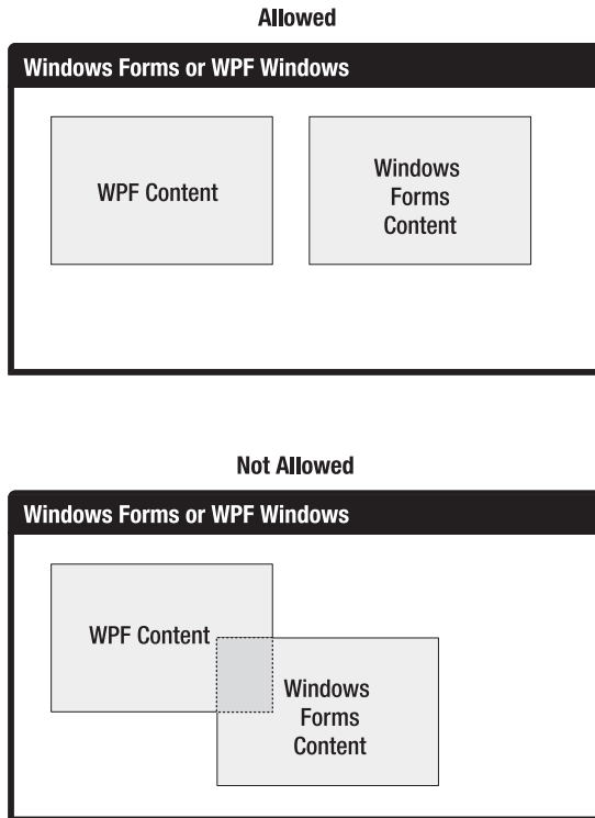
Figure 25-3. The airspace rule
