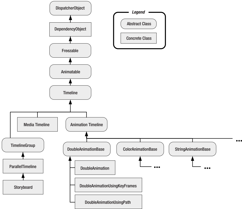
Figure 21-2. The animation class hierarchy
