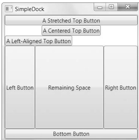
Figure 4-10. Docking multiple elements to the top
