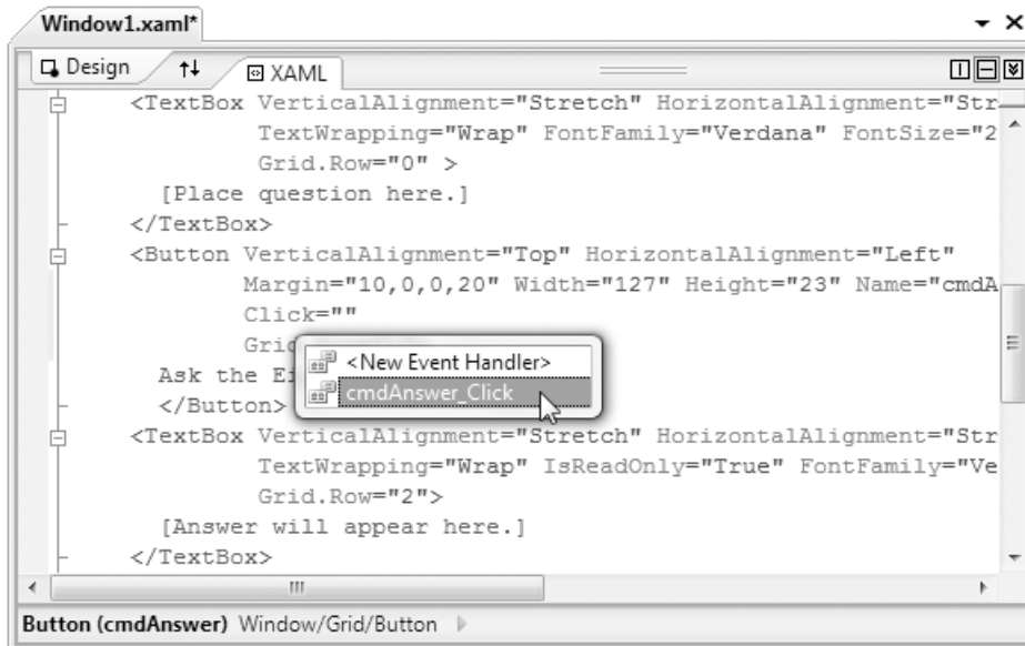
Figure 2-2. Attaching an event with Visual Studio IntelliSense
