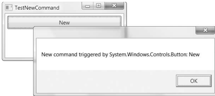
Figure 10-4. A command with a binding
