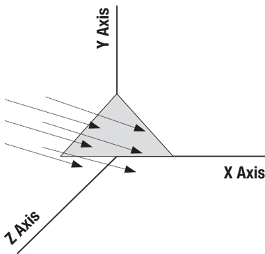
Figure 23-3. The path of a (-1, -1, -1) directional light
