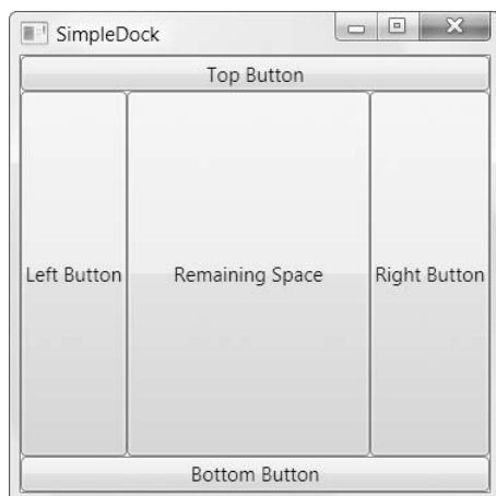
Figure 4-9. Docking to every side
