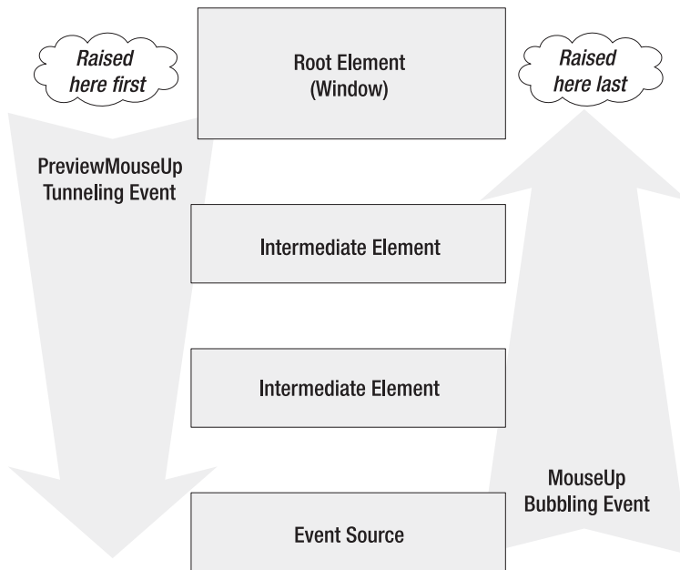
Figure 6-3. Tunneling and bubbling events
