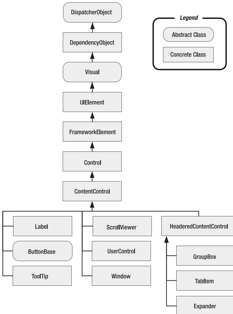
Figure 5-1. The hierarchy of content controls
