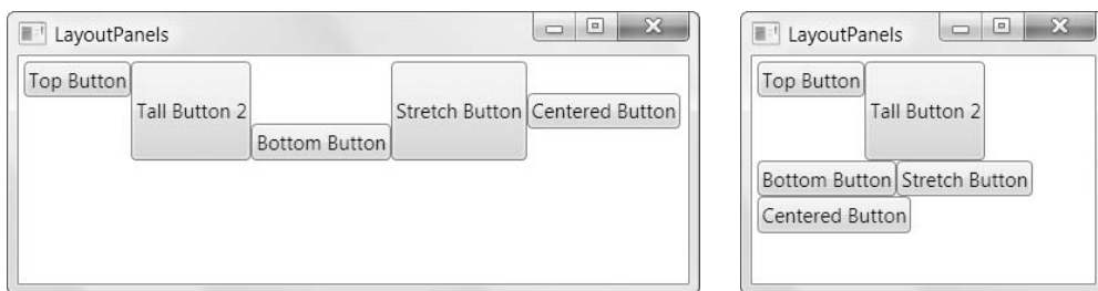
Figure 4-8. Wrapped buttons
