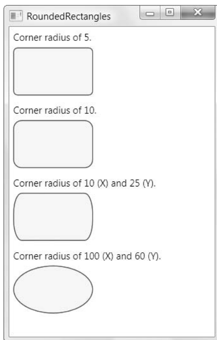
Figure 13-3. Rounded corners
