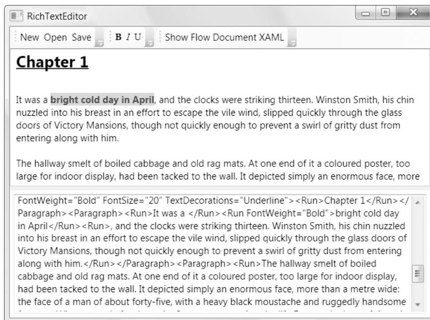
Figure 19-15. Editing text
