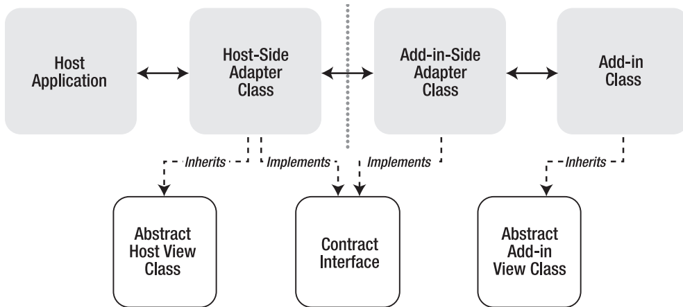
Figure 26-4. Class relationships in the pipeline
