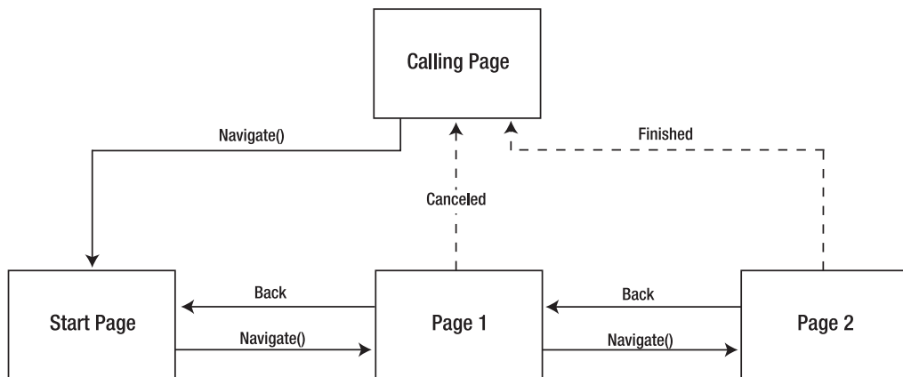
Figure 9-8. Linear navigation
