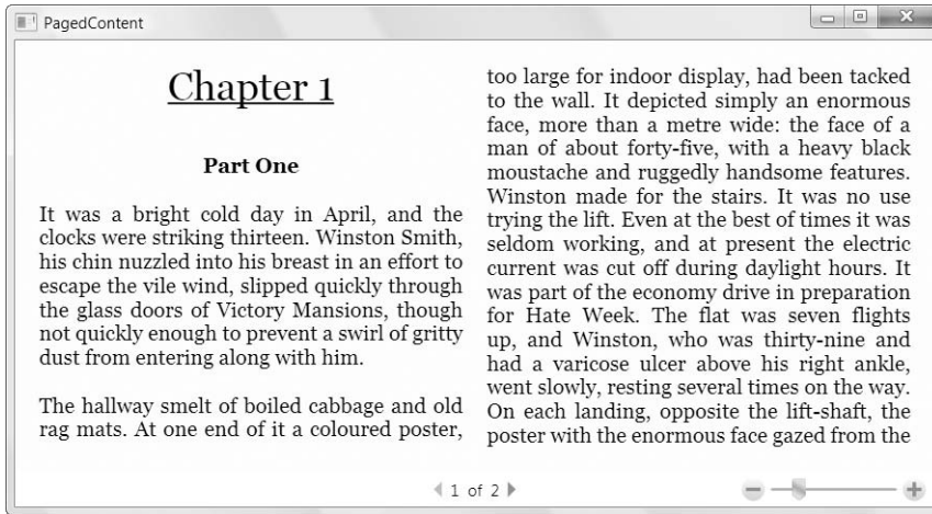
Figure 19-14. Automatic columns
