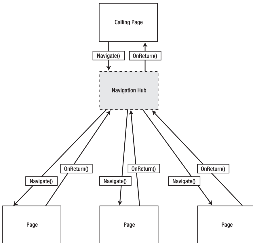
Figure 9-11. Linear navigation
