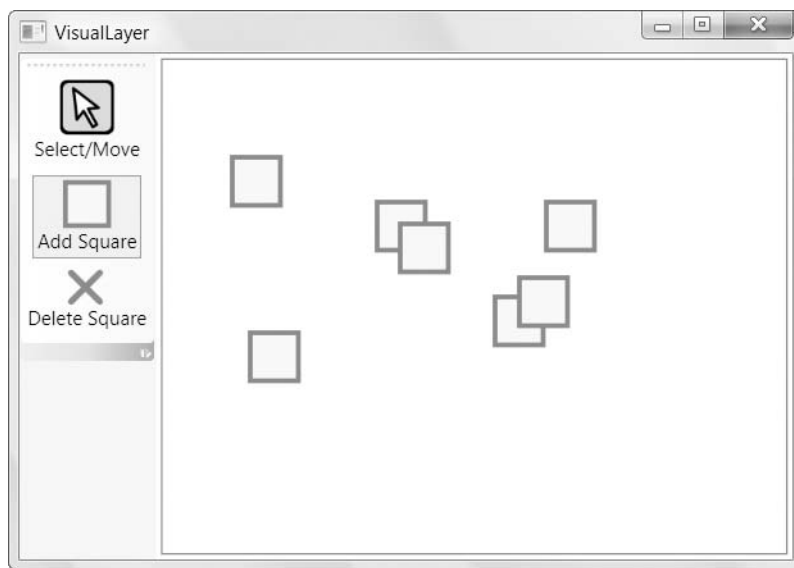
Figure 14-9. Drawing visuals
