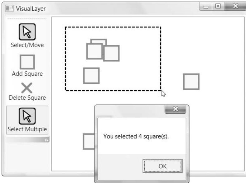
Figure 14-10. Advanced hit testing
