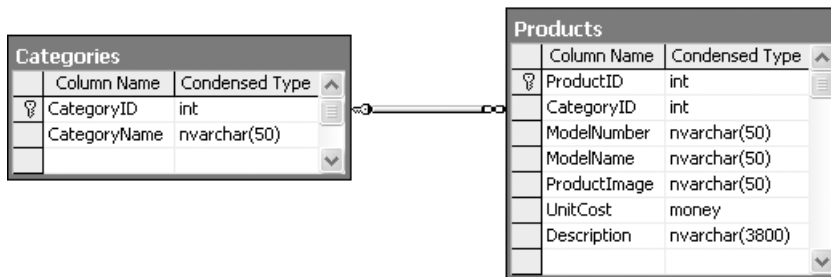
Figure 16-6. A portion of the Store database
