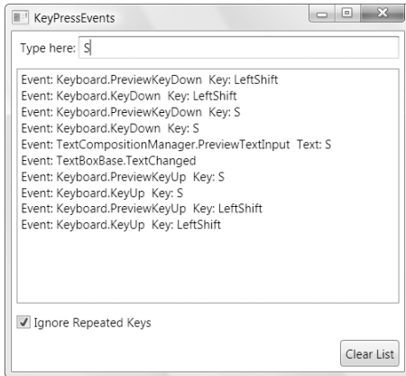
Figure 6-6. Watching the keyboard
