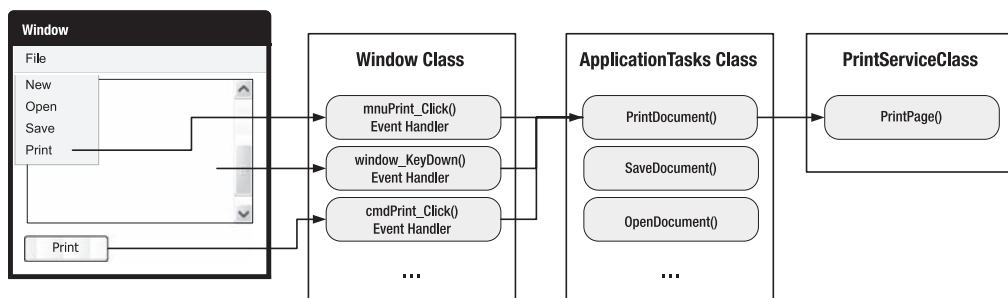
Figure 10-1. Mapping event handlers to a task
