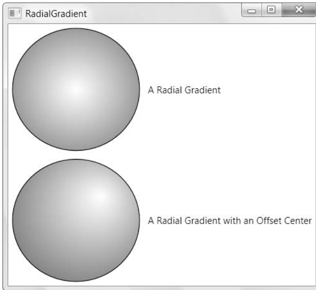
Figure 13-21. Radial gradients
