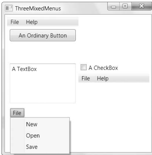
Figure 18-13. Mixed menus
