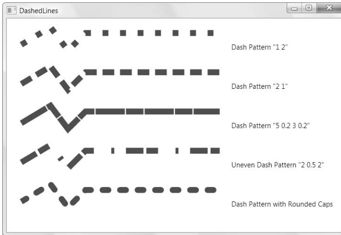
Figure 13-13. Dashed lines
