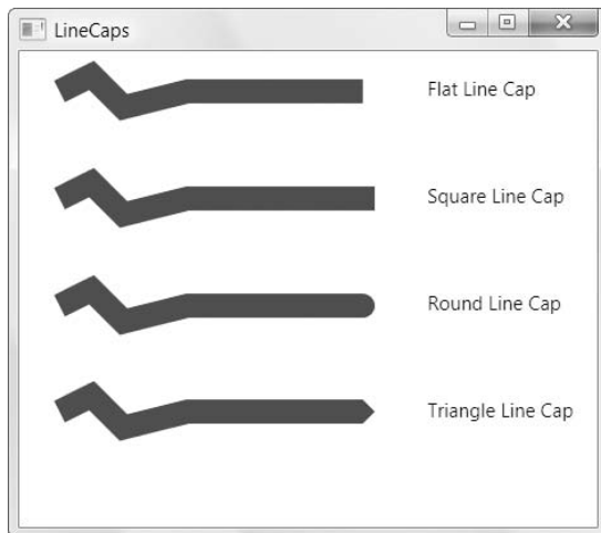
Figure 13-11. Line caps
