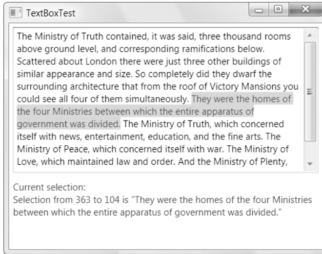
Figure 7-6. Selecting text
