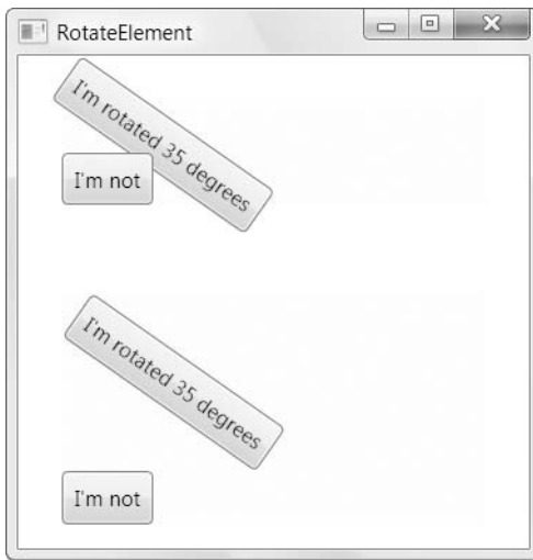
Figure 13-17. Rotating buttons
