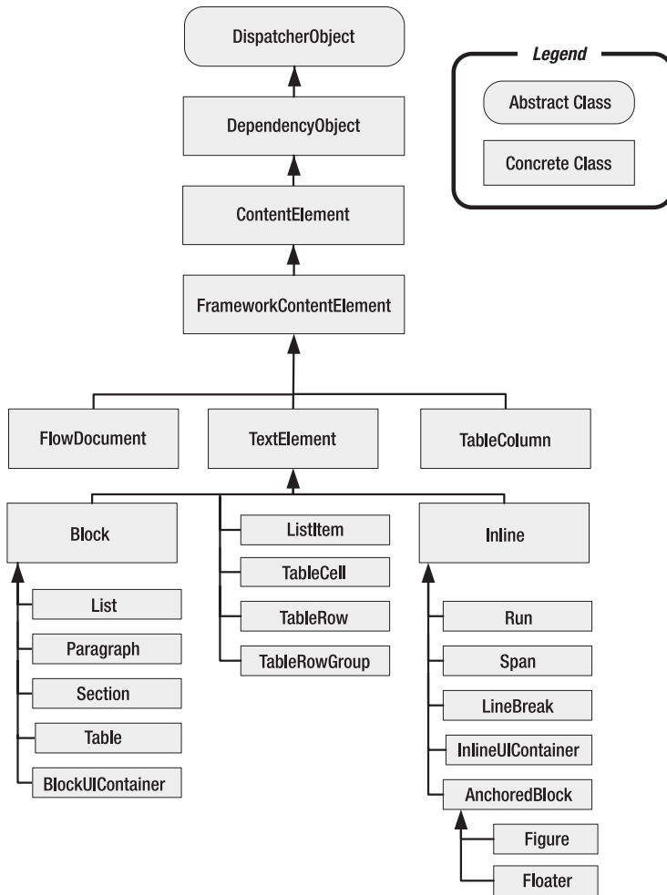
Figure 19-3. Content elements
