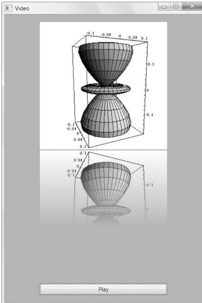
Figure 22-4. Reflected video
