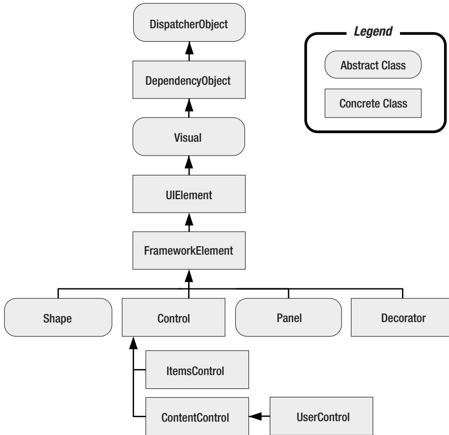
Figure 24-1. Element and control base classes
