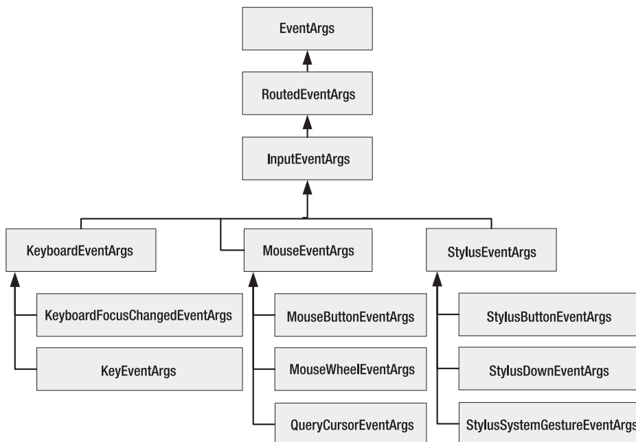
Figure 6-5. The EventArgs classes for input events
