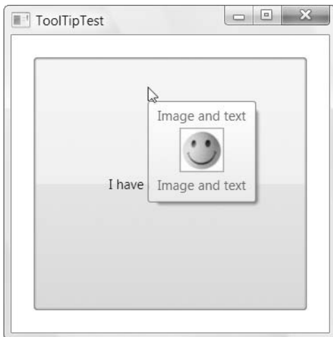
Figure 7-3. A fancy tooltip
