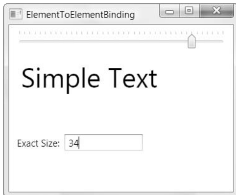
Figure 16-4. Linking two properties to the font size
