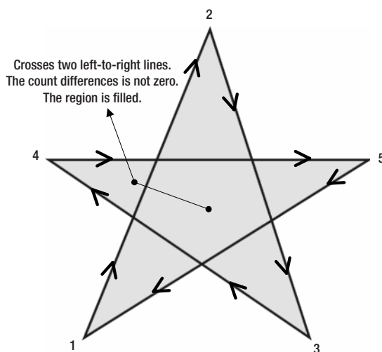
Figure 13-10. Determining fill areas when FillRule is NonZero
