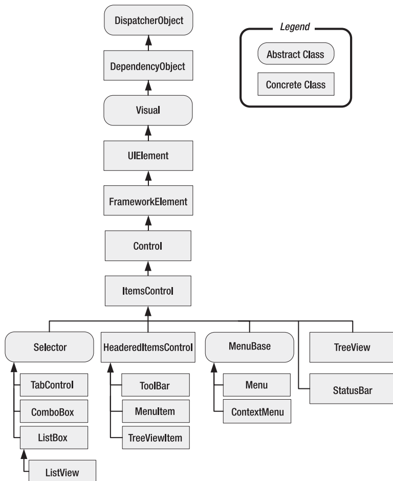
Figure 18-1. Classes that derive from ItemsControl
