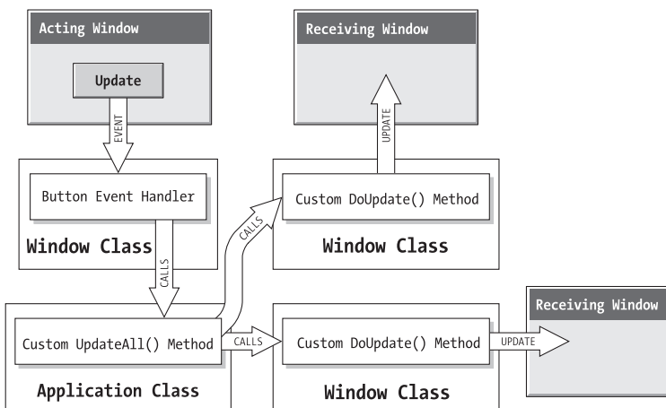
Figure 8-4. A one-to-many window interaction
