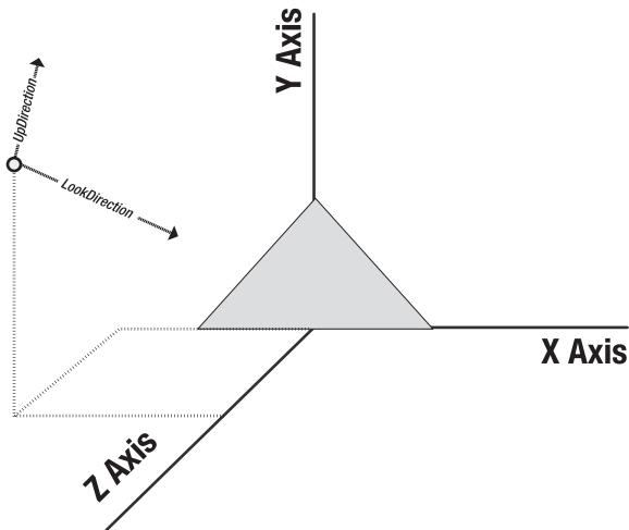
Figure 23-6. Another way to angle the camera
