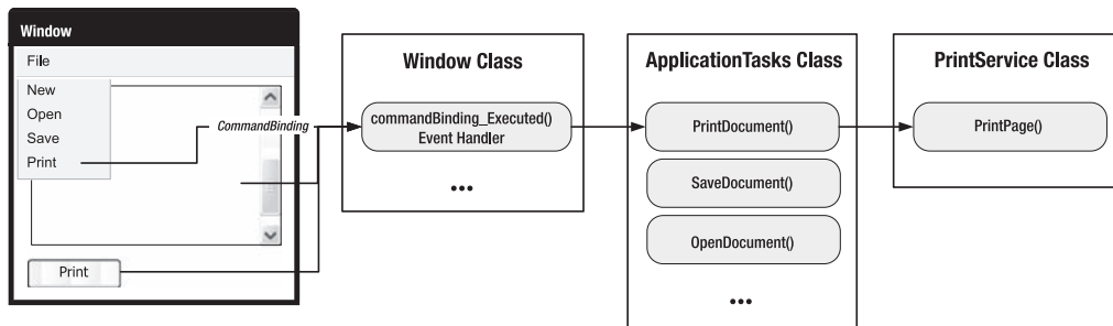
Figure 10-2. Mapping events to a command
