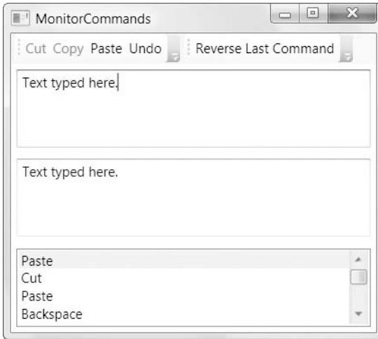
Figure 10-8. An application-wide Undo feature
