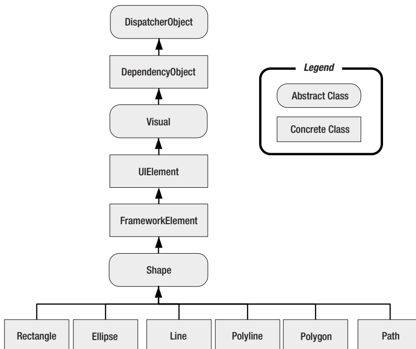
Figure 13-1. The WPF shape classes
