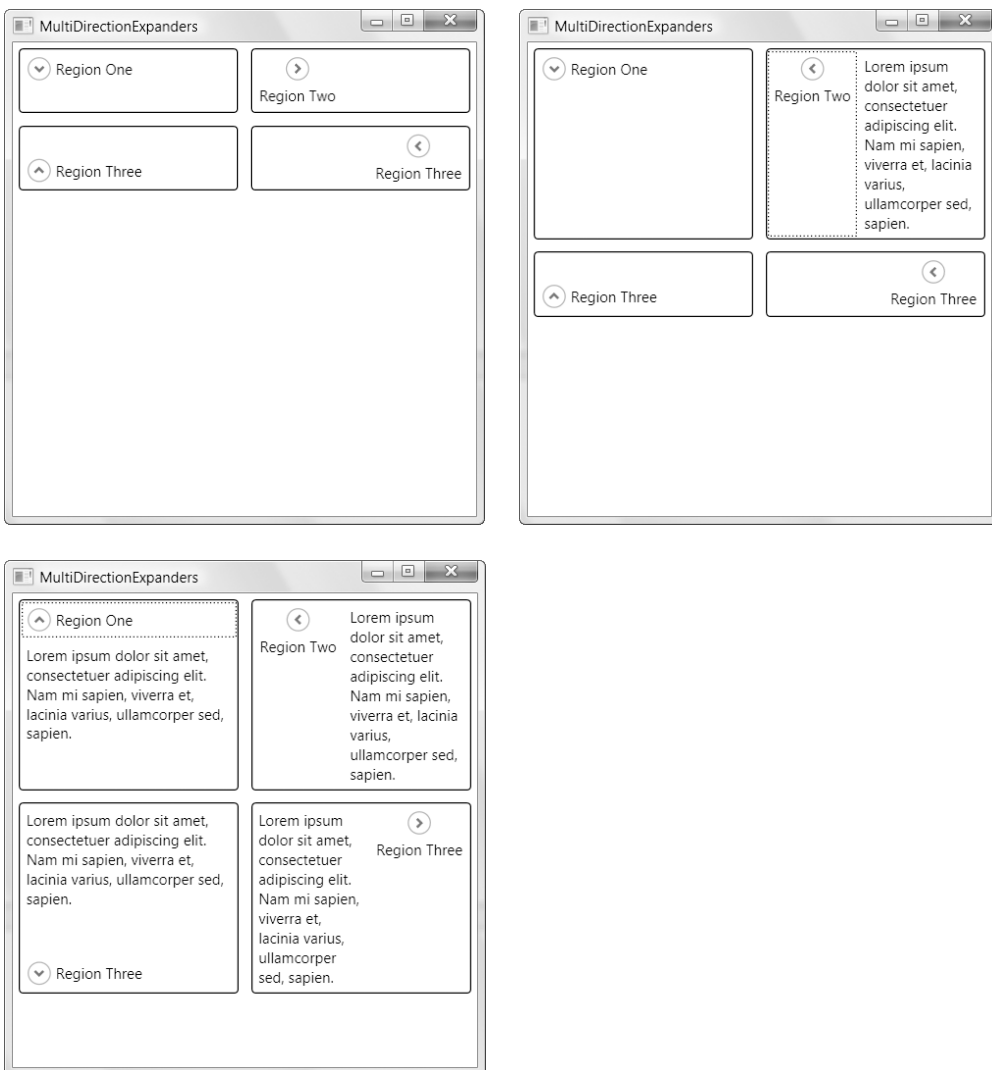
Figure 5-11. Expanding in different directions
