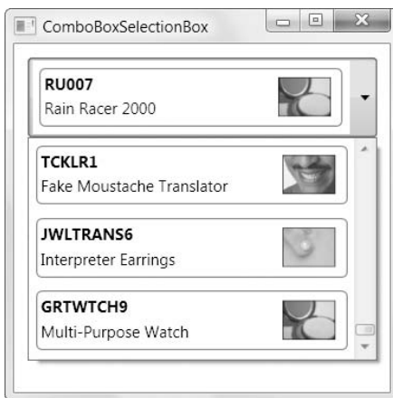
Figure 18-2. A read-only ComboBox that uses templates
