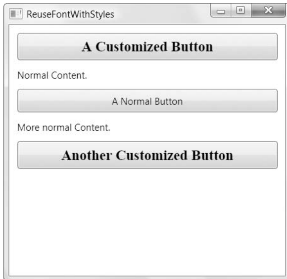
Figure 12-1. Reusing button settings with a style
