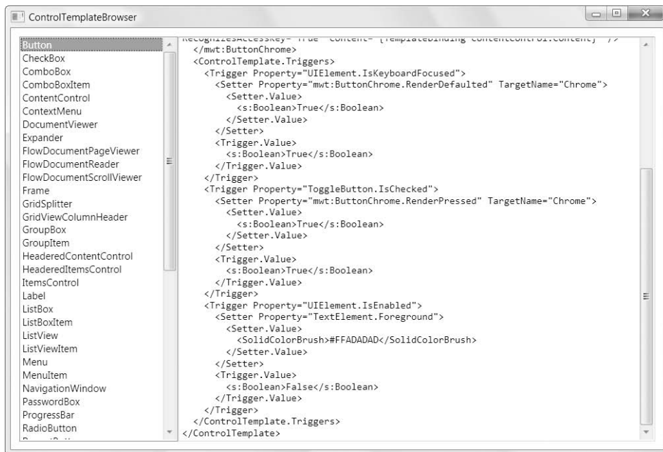
Figure 15-5. Browsing WPF control templates
