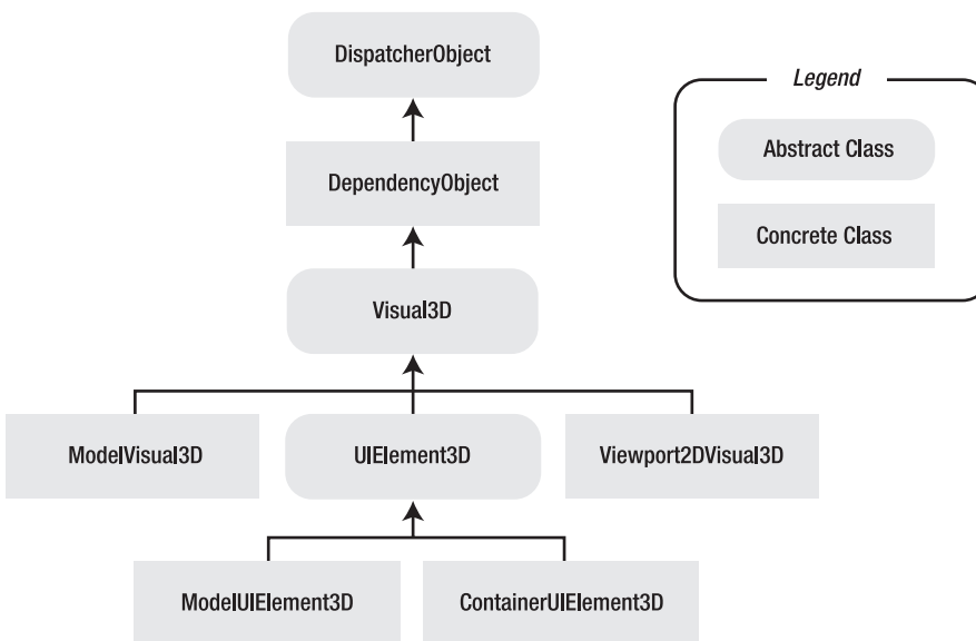
Figure 23-21. The 3-D visual classes
