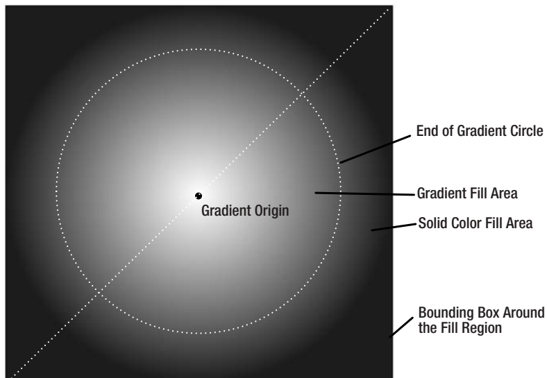
Figure 13-20. How a radial gradient is filled
