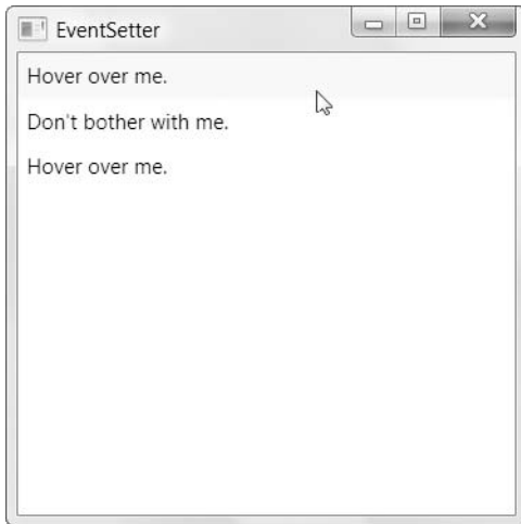
Figure 12-2. Handling the MouseEnter and MouseLeave events with a style
