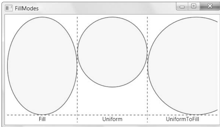
Figure 13-4. Filling three cells in a Grid
