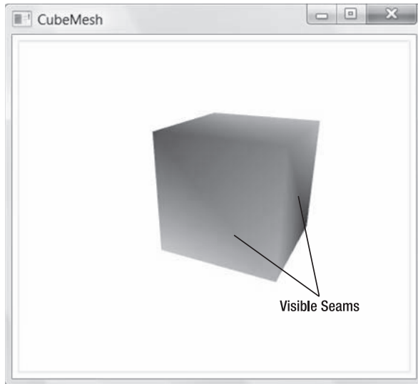
Figure 23-10. A cube with lighting artifacts
