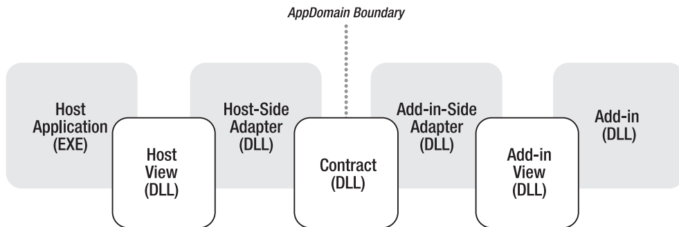
Figure 26-3. Communicating through the add-in pipeline
