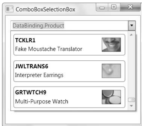
Figure 18-3. An editable ComboBox that uses templates
