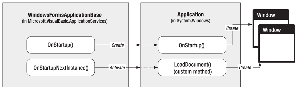
Figure 3-2. Wrapping the WPF application with a WindowsFormsApplicationBase
