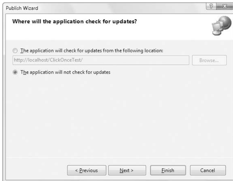
Figure 27-4. Support for automatic updates
