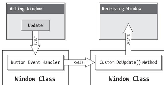
Figure 8-3. A single window interaction
