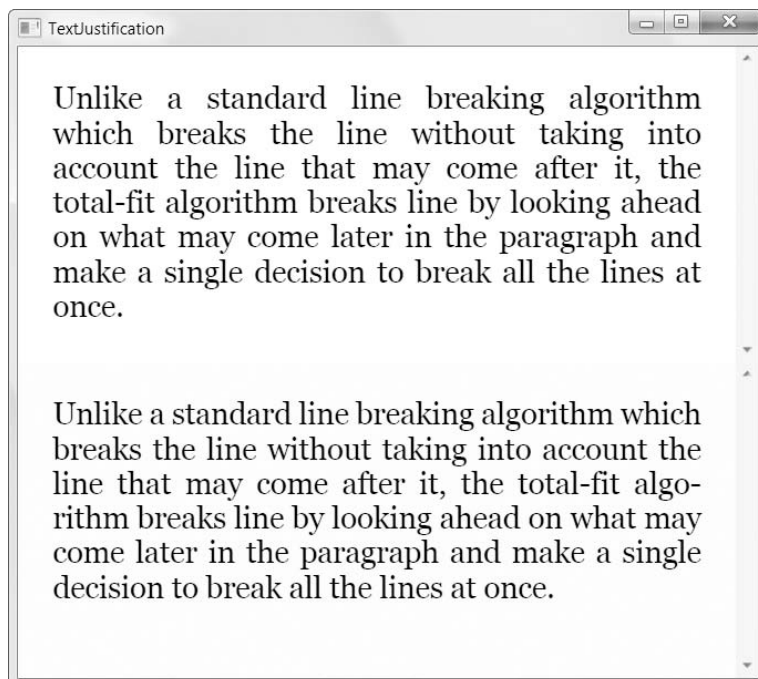
Figure 19-11. Comparing ordinary justification (top) with optimal paragraphs (bottom)
