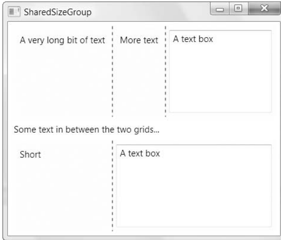
Figure 4-15. Two grids that share a column definition
