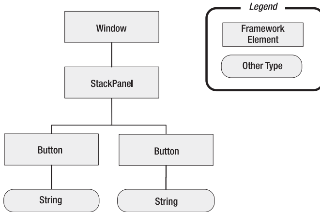
Figure 15-2. The logical tree for SimpleWindow
