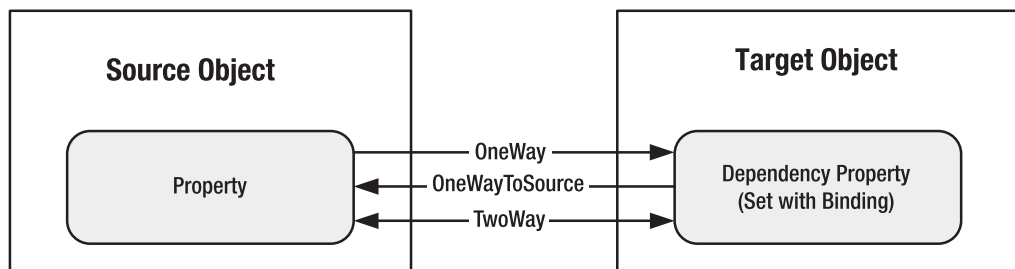
Figure 16-5. Different ways to bind two properties
