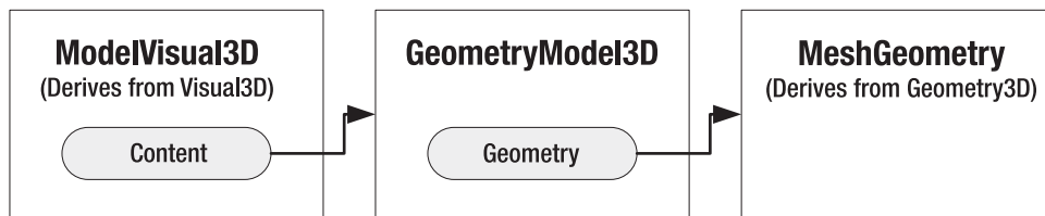
Figure 23-1. How a 3-D object is defined
