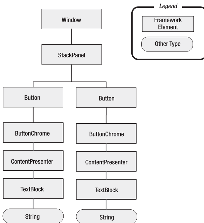
Figure 15-3. The visual tree for SimpleWindow
