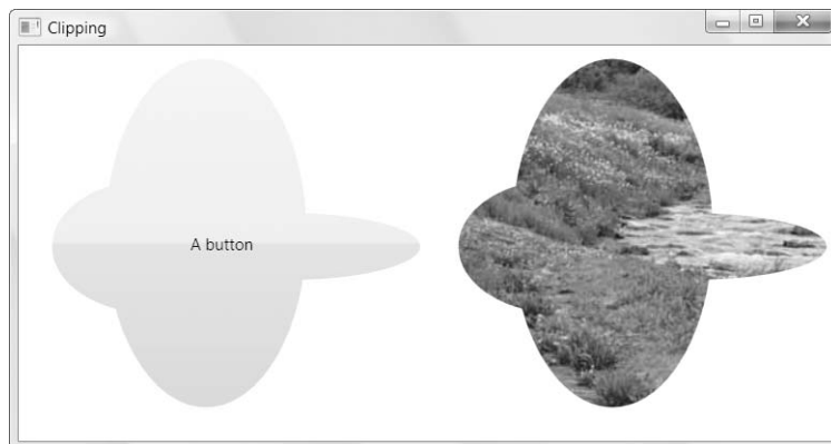
Figure 14-8. Clipping two elements
