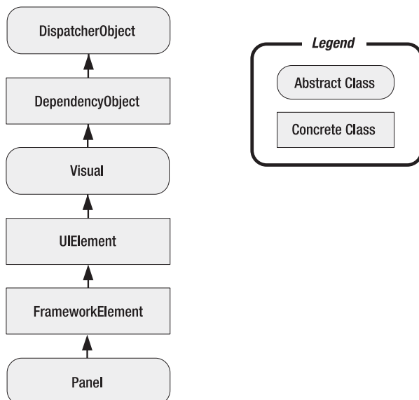
Figure 4-1. The hierarchy of the Panel class
