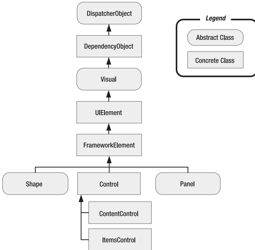
Figure 1-4. The fundamental classes of WPF
