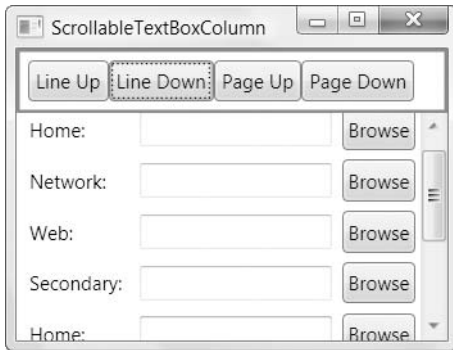
Figure 5-6. Programmatic scrolling
