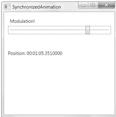
Figure 22-3. Synchronized animations
