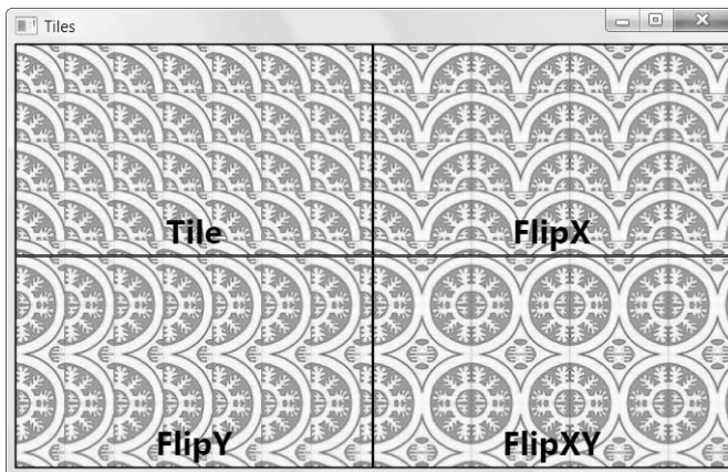
Figure 13-24. Flipping tiles
