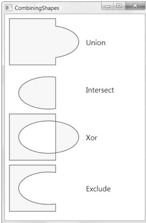
Figure 14-2. Combining shapes
