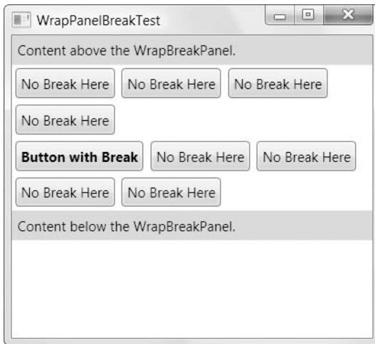
Figure 24-5. The WrapBreakPanel
