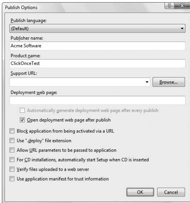
Figure 27-10. Miscellaneous ClickOnce options
