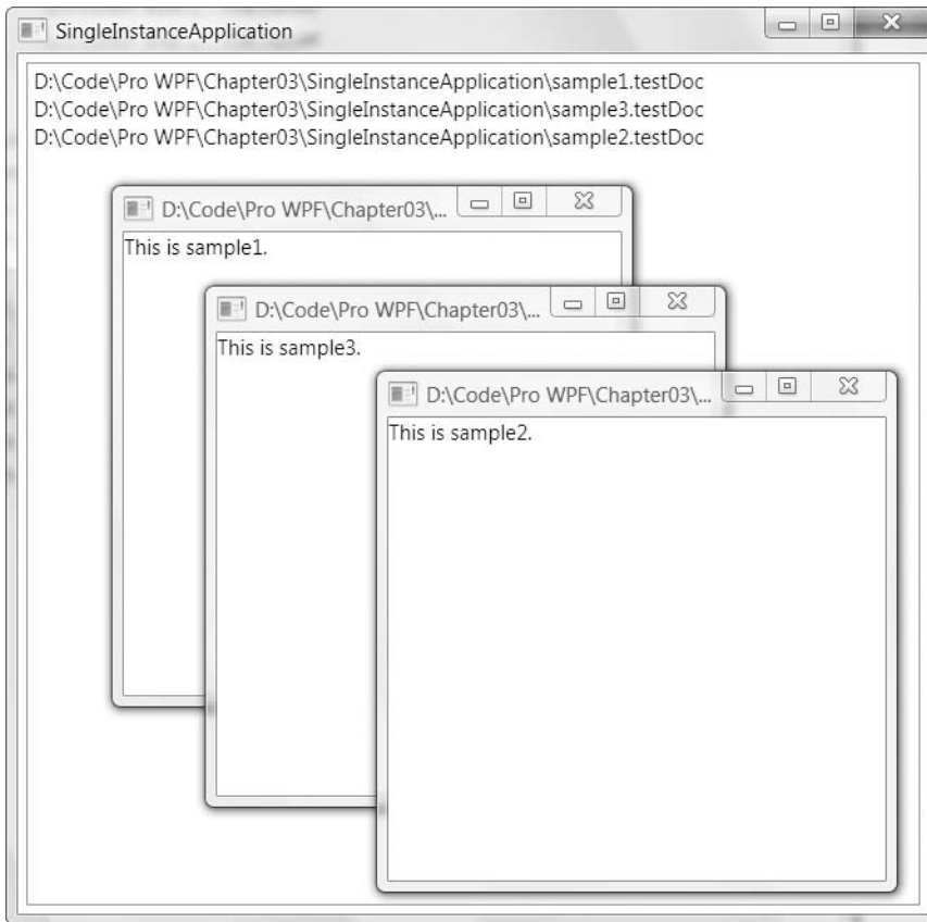
Figure 3-3. A single-instance application with a central window
