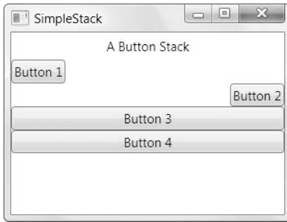
Figure 4-4. A StackPanel with aligned buttons
