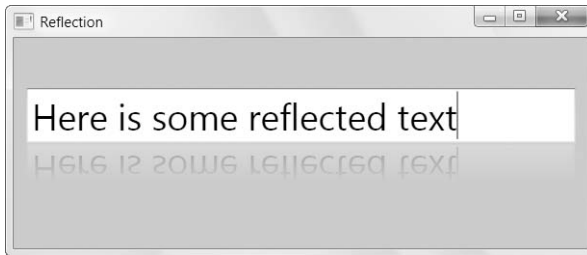
Figure 13-27. VisualBrush + OpacityMask + RenderTransform = reflection effect
