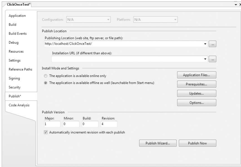
Figure 27-8. ClickOnce project settings
