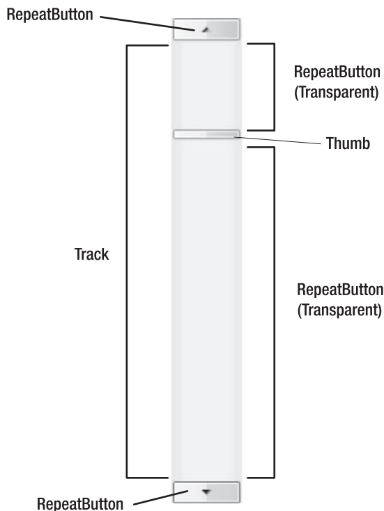
Figure 15-10. Dissecting the scroll bar
