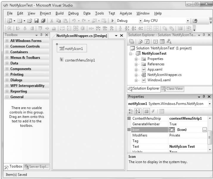
Figure 25-2. The design surface of a component
