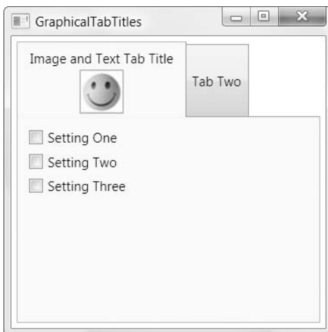
Figure 5-9. An exotic tab title
