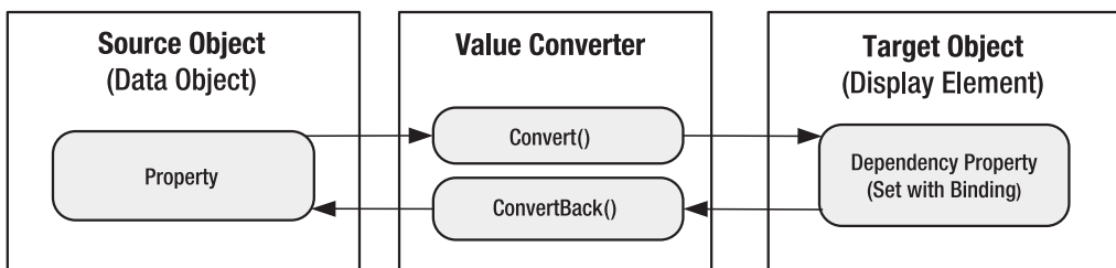
Figure 16-11. Converting bound data
