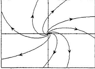
Phase portrait for Problem 36
