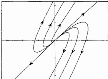
Phase portrait for Problem 21
