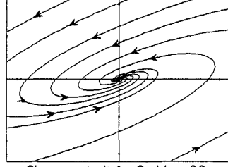
Phase portrait for Problem 38
