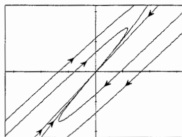
Phase portrait for Problem 20
