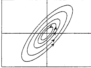
Phase portrait for Problem 37
