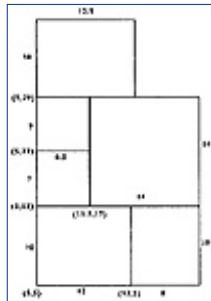
Figure 6.10 The transformed plan
