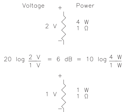
Figure 10.7 Example of the equivalence of voltage and power decibels.
