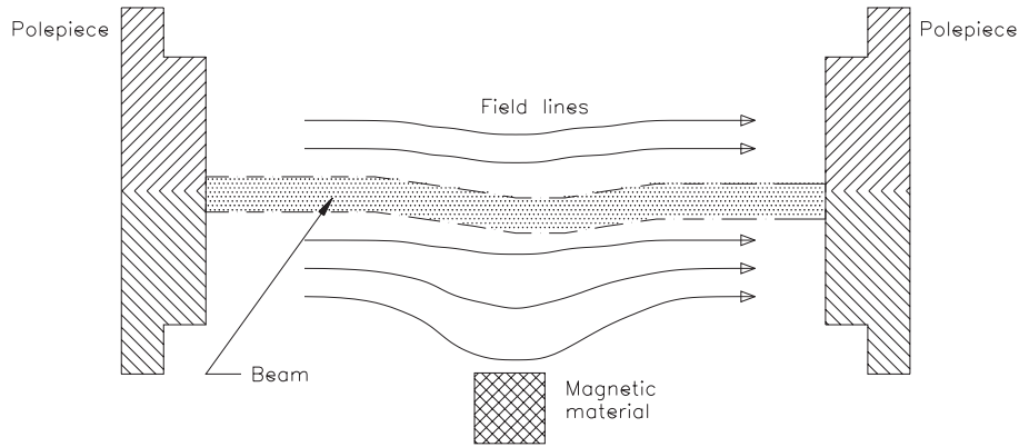
Figure 6.26 Distortion of the field pattern and beam shape due to magnetic material in the magnetic field.
