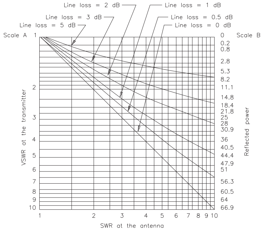
Figure 10.31 Illustration of how the VSWR on a transmission line affects the attenuation performance of the line. Scale A represents the VSWR at the transmitter; scale B represents the corresponding reflected power in watts for an example system.
