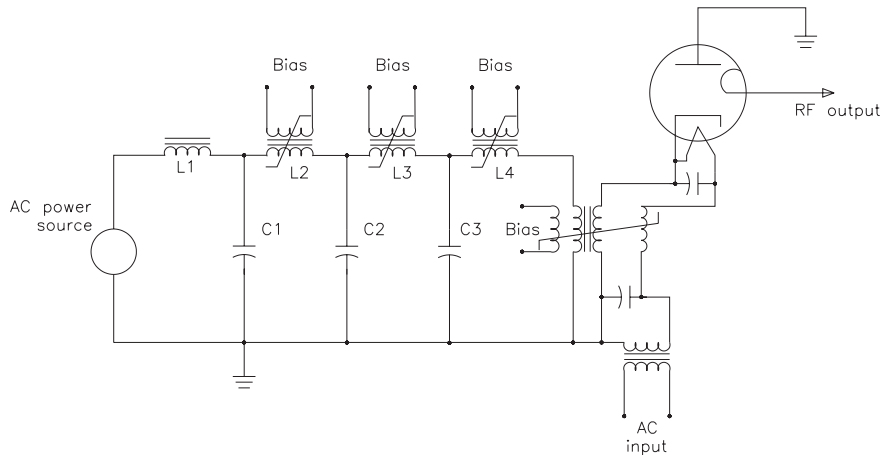
Figure 5.29 A magnetic modulator circuit.
