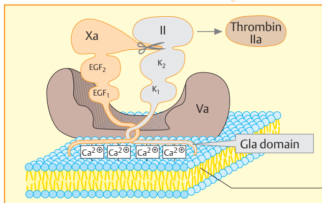
Prothrombinase complex
