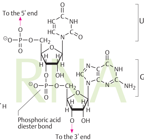
2. RNA (section)
