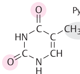
Thymine (Thy)
