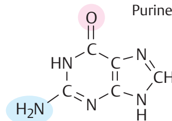
Guanine (Gua)
