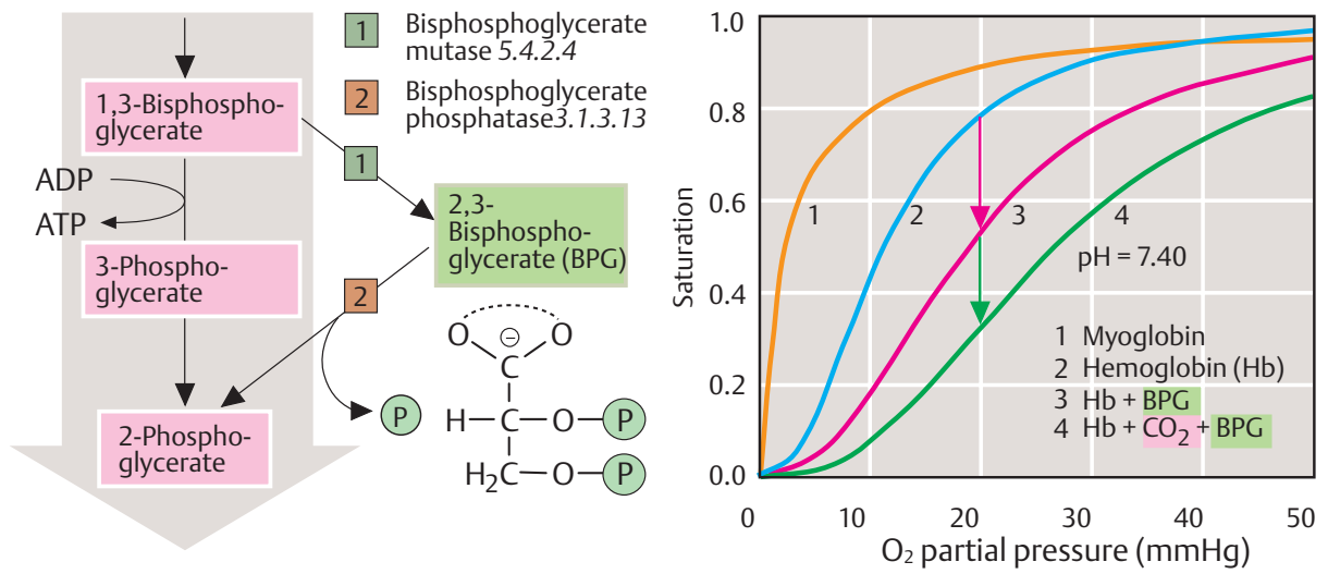
1. BPG metabolism
