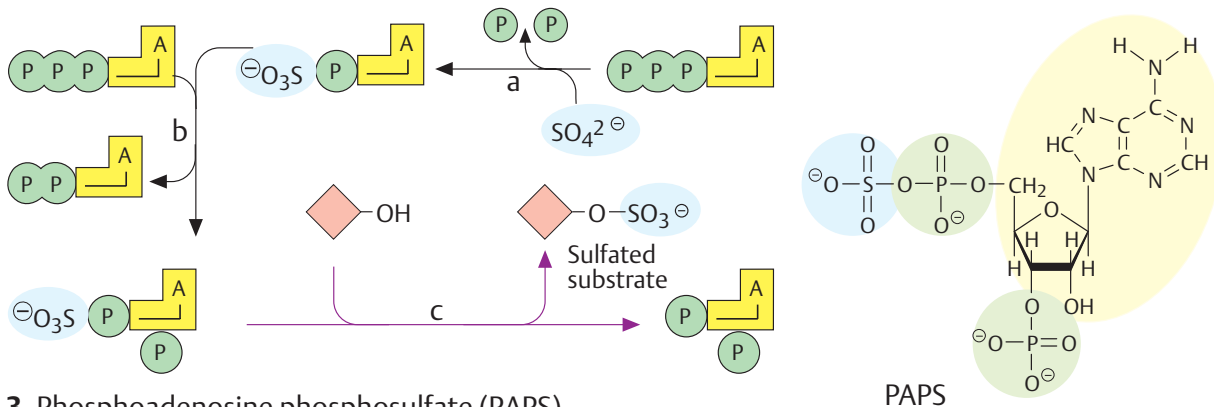
3. Phosphoadenosine phosphosulfate (PAPS)
